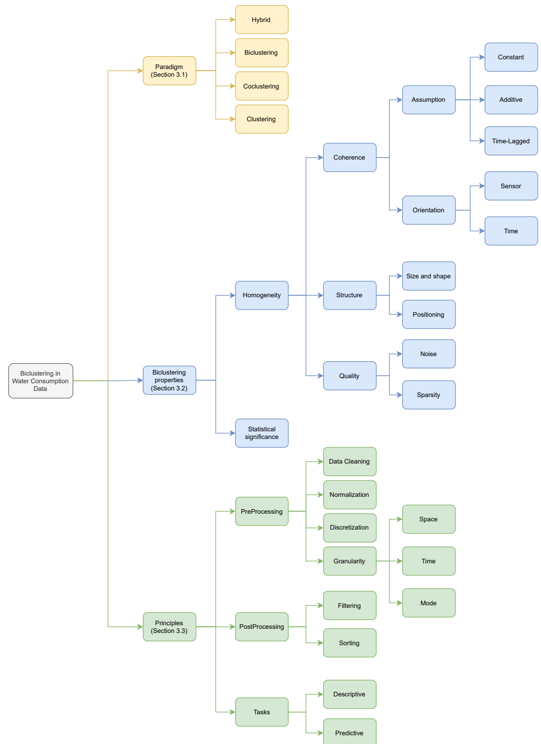
Figure 4. Taxonomy of Biclustering-based data analysis on water demand data: structured view on the major biclustering paradigms, biclustering aspects affecting the analysis, and principles to design and assess biclustering-based approaches.
