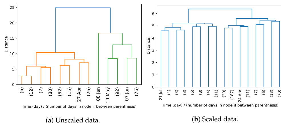
Figure 11. Hierarchical Clustering (Time Dimension) Dendrogram of scaled daily consumption at InfraQuinta, 2017.
