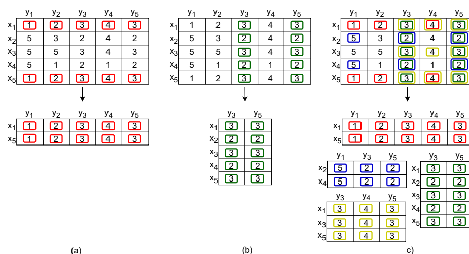
Figure 2. Clustering (a,b) vs. biclustering (c) solutions over an illustrative data matrix.
