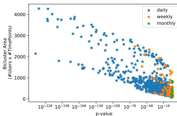
Figure 26. Statistical significance vs. size of biclusters found assuming constant patterns at In-fraQuinta, 2017.
