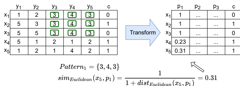
Figure 6. Pattern-centric transformation to map time series data onto multivariate data, obtained by comparing end-users against the found biclusters.
