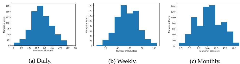
Figure 27. Number of patterns found for each user when combining the biclustering solutions with different pattern assumption at InfraQuinta, 2017.
