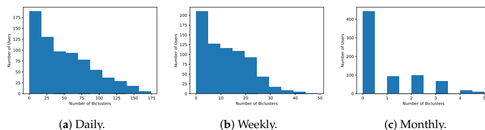
Figure 22. Number of patterns found for each user assuming constant patterns at InfraQuinta, 2017.
