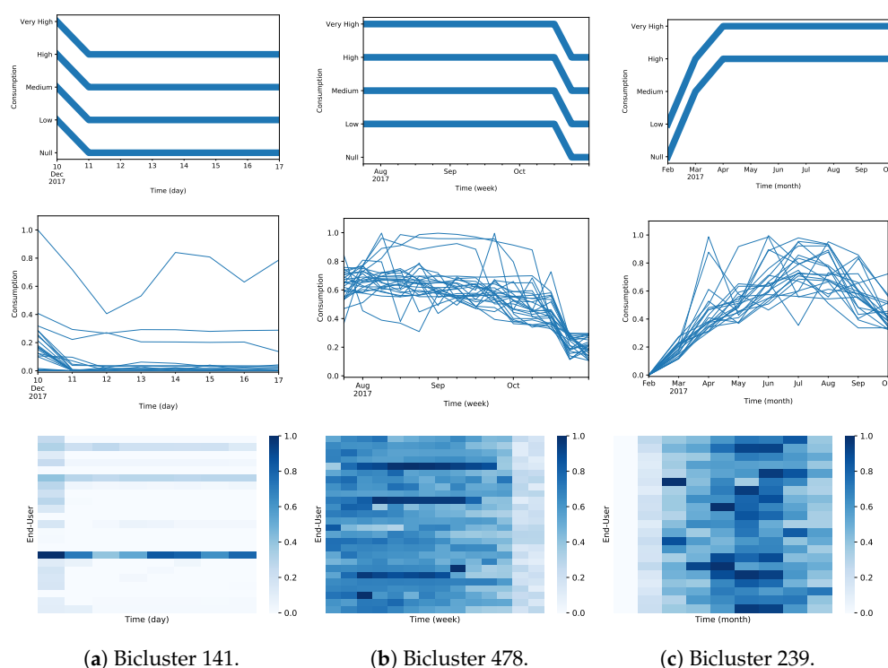
Figure 24. Illustration of the selected biclusters assuming shifting factors (Bicluster 141, Bicluster 478, and Bicluster 239) found on the daily, weekly and monthly dataset. This figure shows the consumption patterns on the first row, the user consumption scaled time series on the second row, and the scaled data heatmap on the third row.
