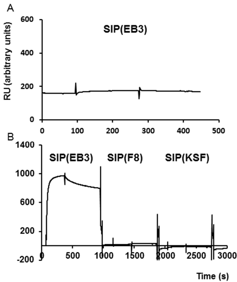
Figure S2. (A) BIAcore profile of SIP(EB3) against the extra domain A of fibronectin coated on the CM5 chip demonstrates absence of binding. (B) BIAcore profiles of SIP(EB3), SIP(F8) and SIP(KSF) antibodies against DLK1-Fc fusion protein coated on the CM5 chip, respectively.
