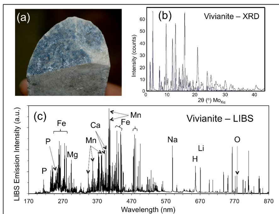
Figure 8. (a) Fine-grained vivianite [\text{Fe}_3(\text{PO}_4)_2 \cdot 8\text{H}_2\text{O}] on a fracture in drill core 18-BD-288 from the Carolina Lithium Project prospect in Gaston County, N.C.; (b) X-ray diffraction pattern (Mo K\alpha radiation) of vivianite after background subtraction (black), with International Centre for Diffraction Data pattern matches shown by vertical blue bars; and (c) handheld LIBS spectrum of vivianite showing the prominent P peaks at 213.62, 214.92, and 255.32 nm and the major Li peak at 670.79 nm. The suite of weak unlabeled peaks in the ultraviolet and visible portions of the LIBS spectrum between 234–278 nm and 404–441 nm are Fe emissions. The unlabeled peaks in the infrared portion of the LIBS spectrum between 700–870 nm are for the Ar purge gas used for the LIBS analysis. The very strong H peak at 656.3 nm in this spectrum, compared to those shown in Figures 6 and 7, indicate that this sample is a hydrated mineral and further supports its identification as vivianite.
