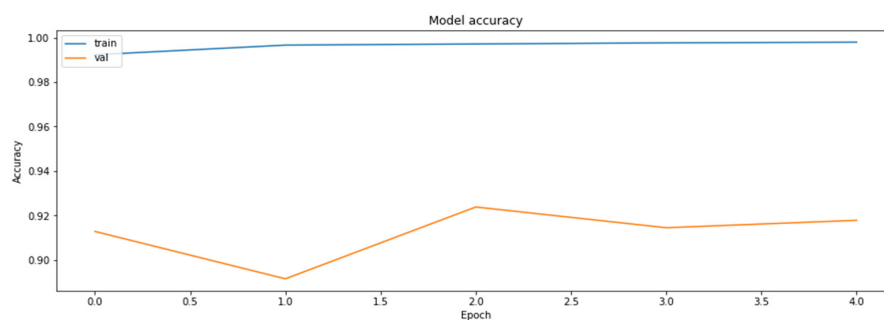
Figure A4. The accuracy of the model for the training and the validation datasets obtained during the training of the model with the weights clustered with the linear initialization of 32 centroids.
