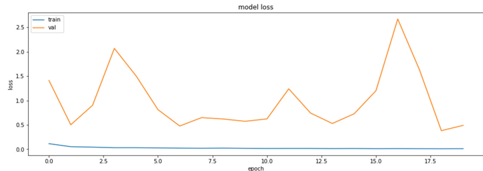
Figure 1. The loss function values for the training and the validation datasets obtained based on RestNet18 model.
