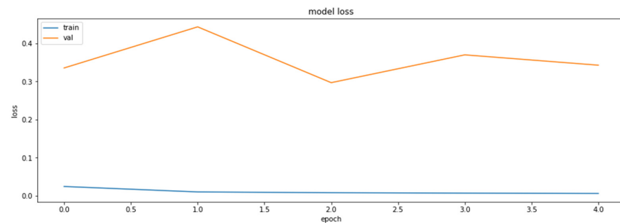
Figure A3. The loss function values for the training and the validation datasets obtained during the training of the model with the weights clustered with the linear initialization of 32 centroids.
