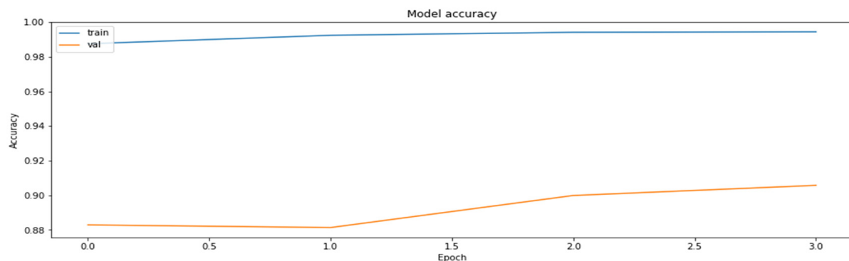
Figure 8. Training and the validation datasets obtained during the application of the pruning part of the PCQAT.
