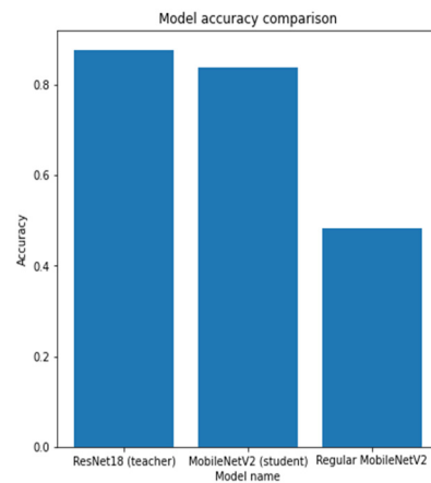
Figure 17. The comparison of the accuracy of the teacher model (the base ResNet18 model), the student model (MobileNetV2), and the regularly trained student model (MobileNetV2).
