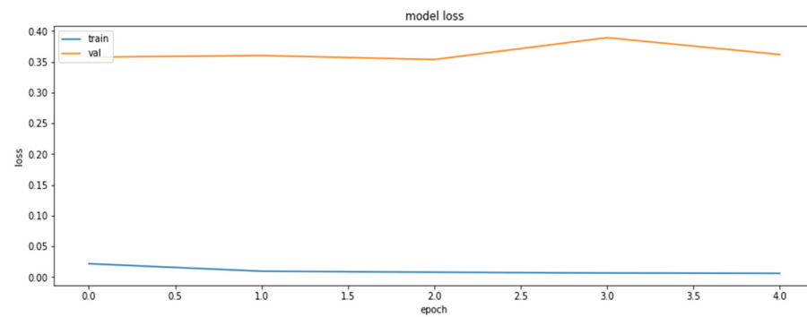
Figure A1. The loss function value for the training and the validation datasets obtained during the training of the model with the weights clustered with the KMeans++ initialization of 32 centroids.
