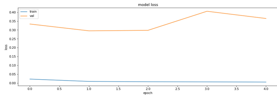
Figure A5. The loss function value for the training and the validation datasets obtained during the training of the model with the weights clustered with KMeans++ initialization of 256 centroids.
