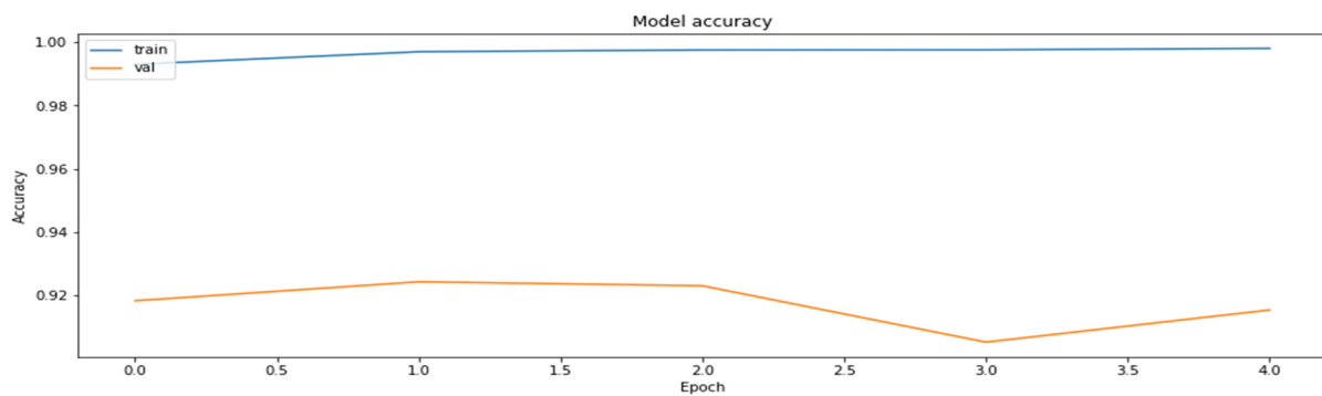
Figure A6. The accuracy of the model for the training and the validation datasets obtained during the training of the model with the weights clustered with KMeans++ initialization of 256 centroids.
