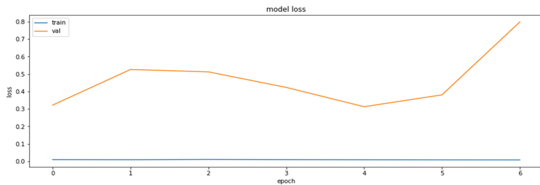
Figure 11. The loss function values for the training and the validation datasets based on QAT part of the PCQAT method.
