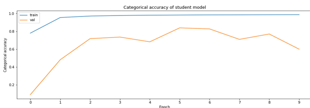
Figure 14. The accuracy of the model for the validation datasets obtained during the model distillation process.
