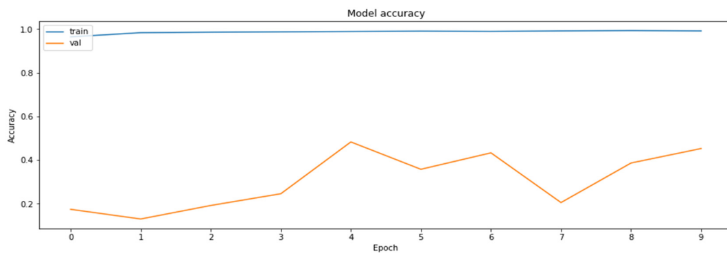
Figure 16. The accuracy of the model for the validation datasets obtained during the regular training of the model.
