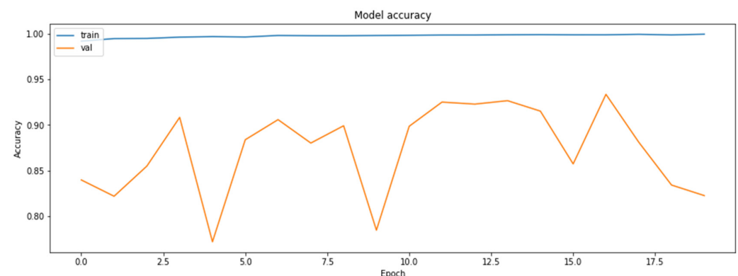
Figure 4. The accuracy of the model on the training and the validation datasets by polynomial iterative model.
