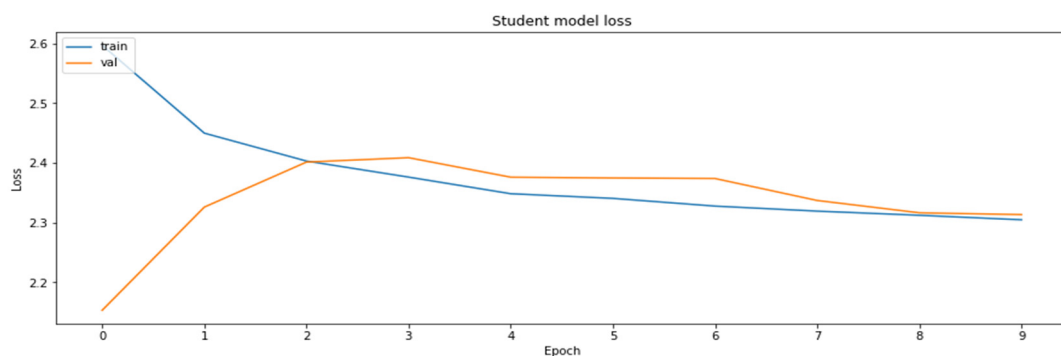
Figure 13. Training and the validation datasets obtained during the model distillation process.
