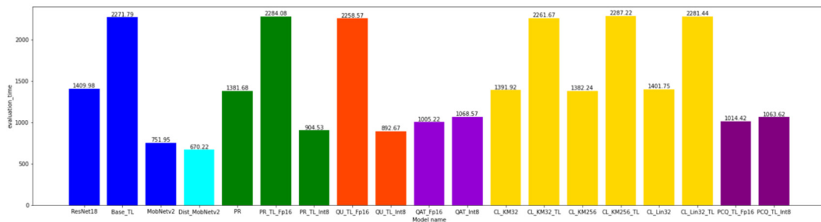
Figure A7. The comparison of the model accuracies and the comparison of the model execution time.
