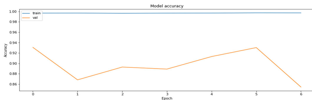
Figure 12. The accuracy of the model for the training and the validation datasets based on the QAT part of the PCQAT method.
