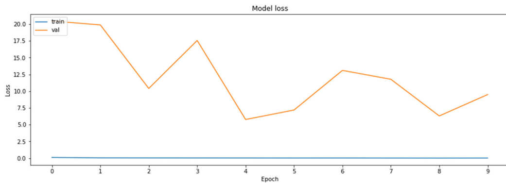
Figure 15. The loss function values for the validation datasets obtained during the regular training of the model.
