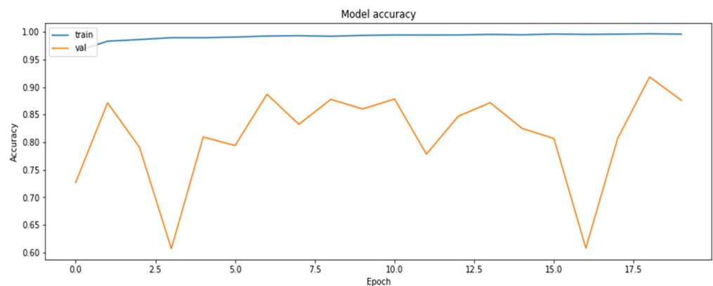
Figure 2. The accuracy of the model for the training and the validation datasets obtained based on RestNet18 model.
