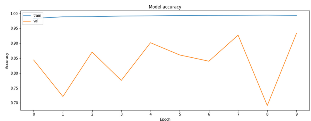
Figure 6. The accuracy of the model on the training and the validation datasets obtained during the training with the application of the QAT method.
