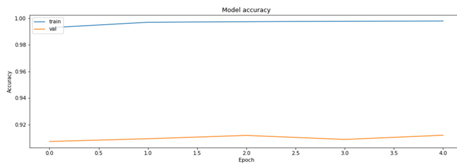
Figure A2. The accuracy of the model for the training and the validation dataset obtained during the training of the model with the weights clustered with KMeans++ initialization of 32 centroids.
