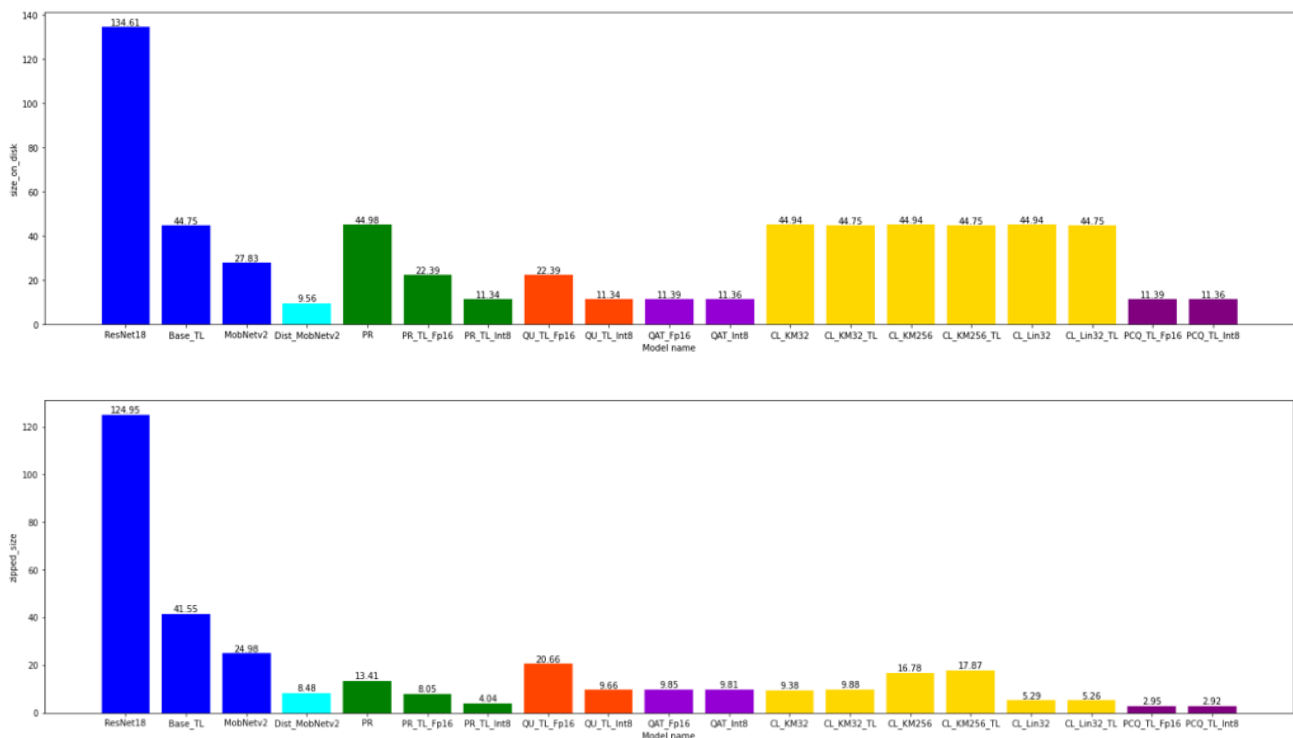
Figure A8. The comparison of the model size on the disk and the comparison of the model size on the disk after the application of the zip function.
