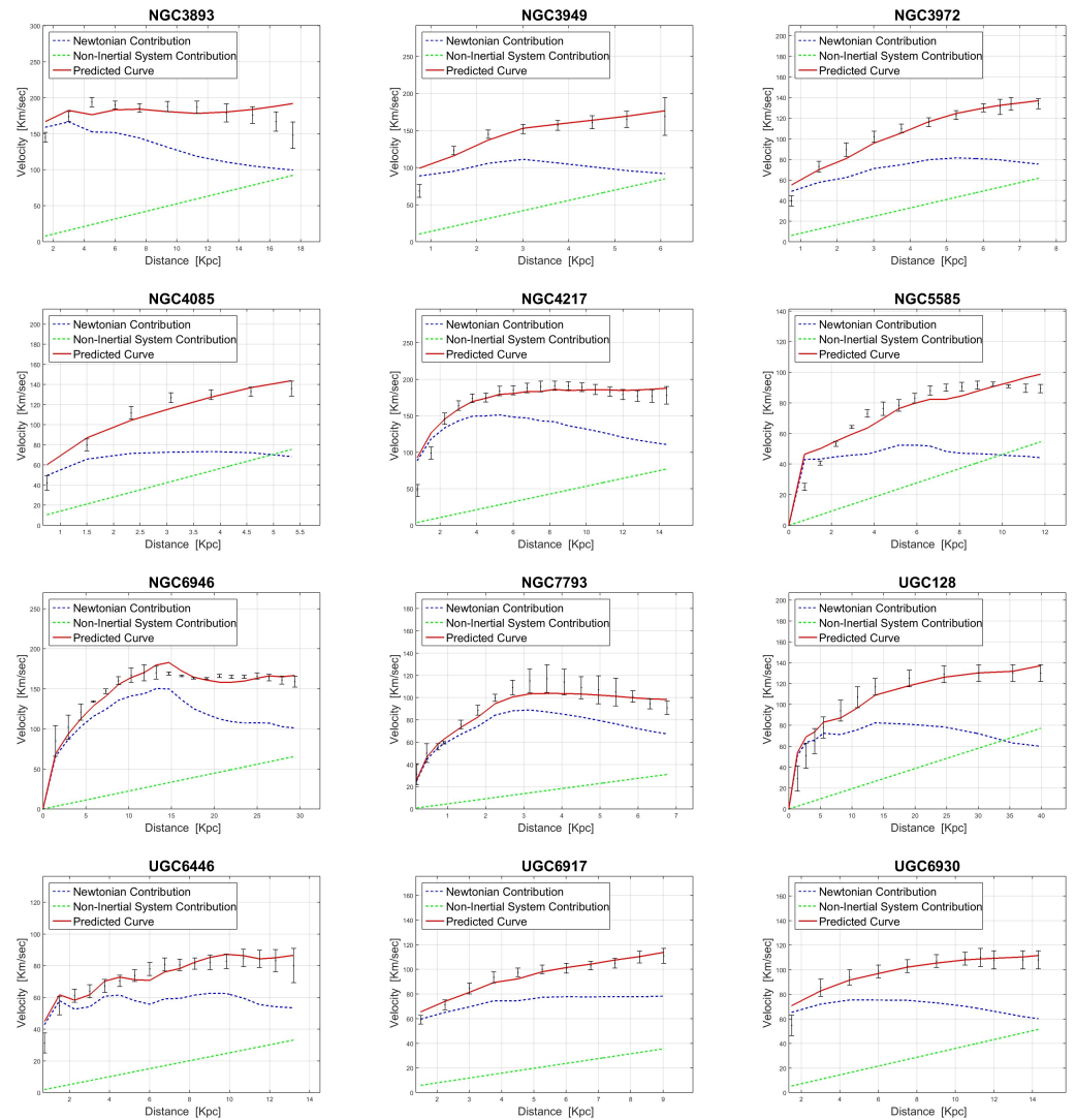
Figure A3. RCs for the different galaxies are presented. In each panel one can see the measured values (black error bars) together with the predicted curve (red line). The dashed blue curve corresponds to the Newtonian term v_k(r) while the dashed green line corresponds to the linear correction term \omega r .
