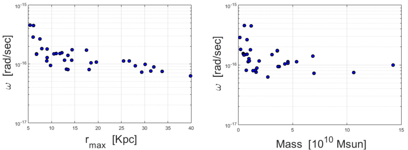
Figure 5. Left panel: a scatter plot of the best-fitted \omega 's vs. r_{max} (the last point of the RC). Right Panel: a scatter plot of \omega vs. the galaxy's mass. Both plots were produced using the sample of galaxies summarized in Appendix B.
