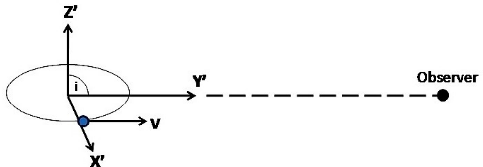
Figure A1. A stationary distant observer is located on the y' - axis (i.e., v_{sys} = 0 , \sin(i) = 1 ). Such an observer would measure a value of V for the line of sight velocity, thus, relying on relation (A1), would extract a value of V for the rotational velocity. As can be seen in the figure, this value is valid relative to the system K' . At any other frame which is rotating relative to K' , the rotational velocity would take a different value.
