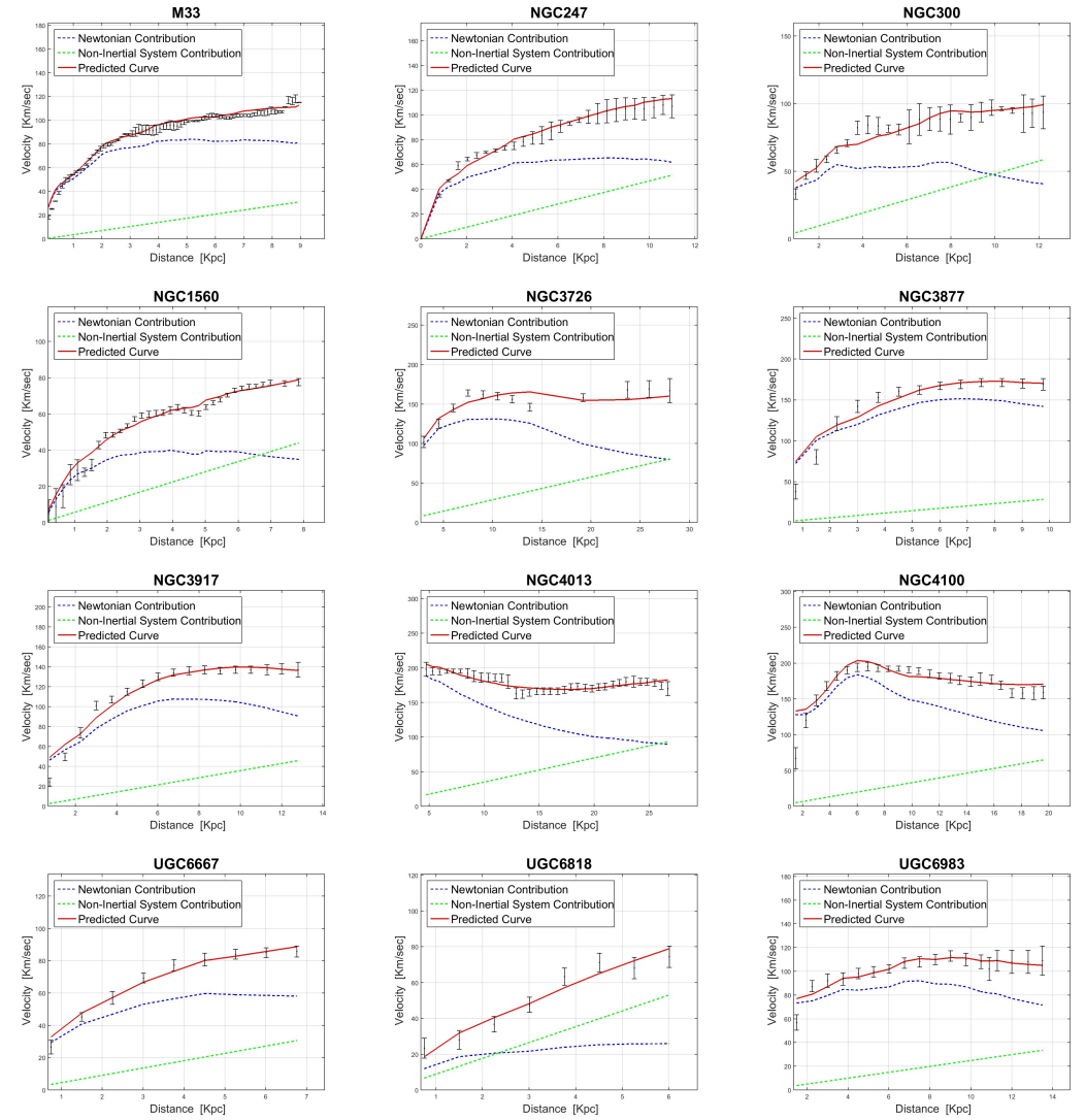
Figure A2. RCs for the different galaxies are presented. In each panel one can see the measured values (black error bars) together with the predicted curve (red line). The dashed blue curve corresponds to the Newtonian term v_k(r) while the dashed green line corresponds to the linear correction term \omega r .
