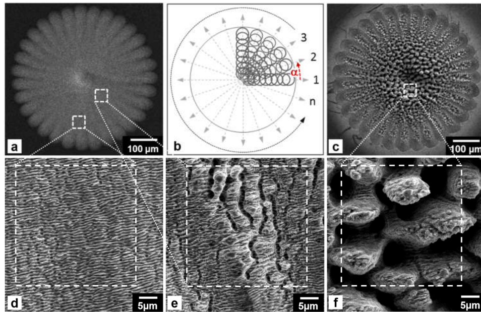
Figure 6. SEM micrographs showing ripple (a) and cone-like protrusion (CLP) (c) surface textures produced on stainless steel; the direct-write scanning procedure for the radial matrices as used for tightly mapping a variable set of pulse overlaps (b); magnified view on low spatial frequency LIPSS (LSFL) (d), micro grooves and spikes (e) as well as CLPs (f) originating at low and high peak fluence pulses of 0.7 \text{ J/cm}^2 and 3.7 \text{ J/cm}^2 .
