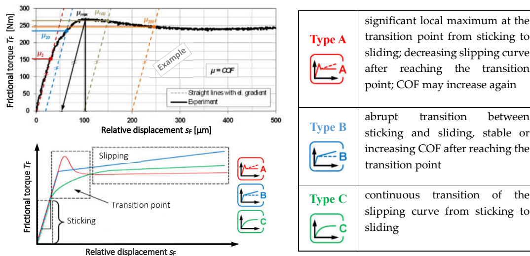
Figure 5. Exemplary illustration of the evaluation methods applied to determine the static coefficient of friction (COF) also seen in Table 2 ( \mu_{20} , etc.). Three types of friction can be distinguished depending on the torque progression curve schematically shown bottom, left. A detailed description of the different friction types is provided in the table on the right.
