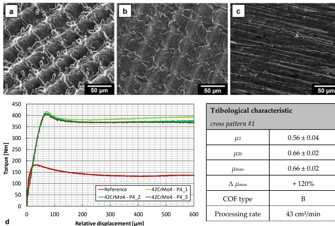
Figure 13. SEM micrographs showing the cross pattern made with 2 scan passes (a) before and (b) after friction testing and (c) the counter body surface after the friction test; the recorded slipping
