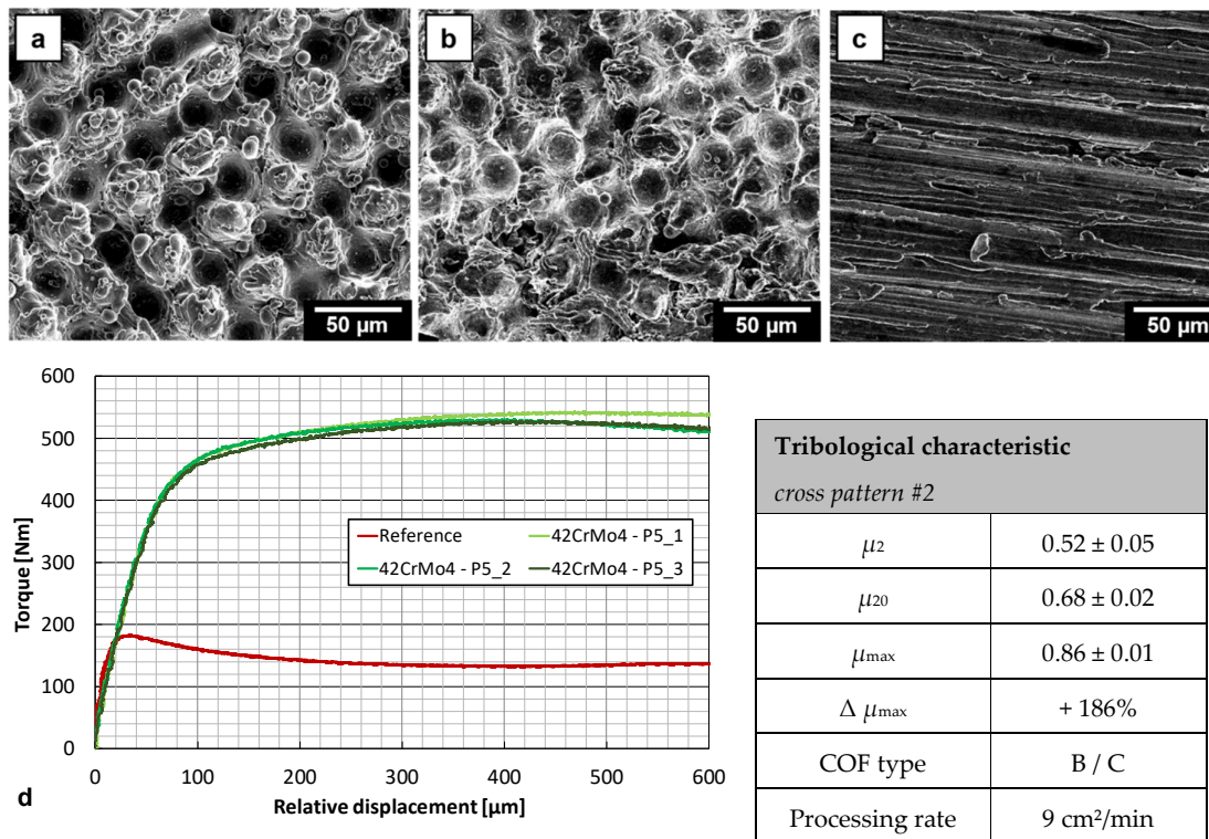
Figure 14. SEM micrographs showing the cross pattern made with 10 scan passes (a) before and (b) after friction testing and (c) the counter body surface after the friction test; the recorded slipping curves (d) and a summary of the tribological characteristic of the cross pattern texture are presented (table bottom, right).
