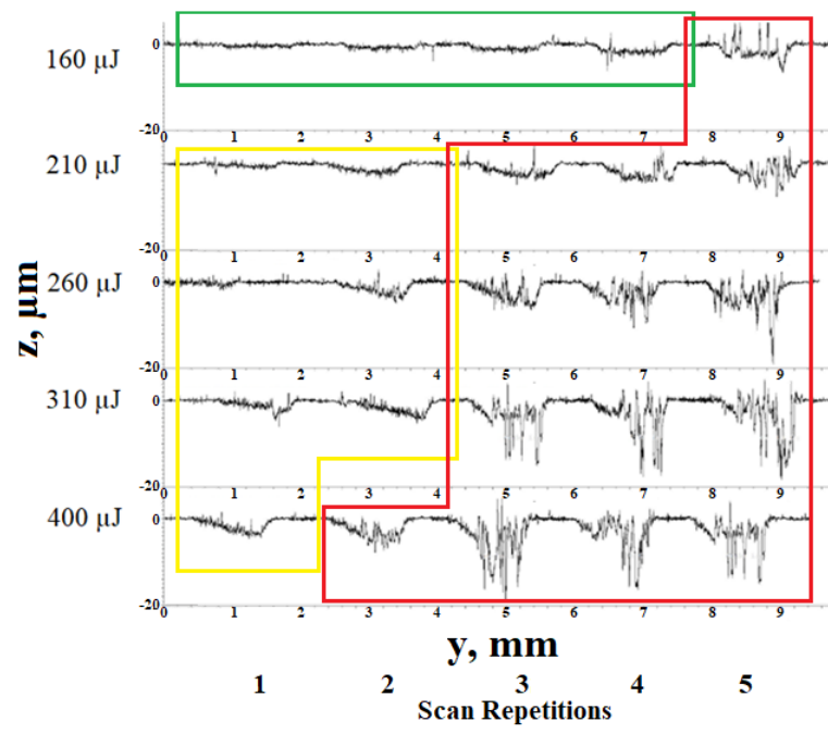
Figure S1. Profiles of laser treated areas.
