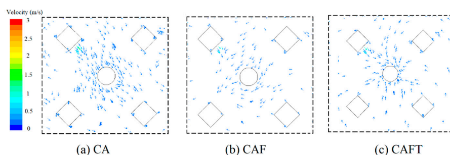
Figure 7. The velocity vector of airflow near the infected occupant under different ventilation conditions ( Z = 1.1 m).
