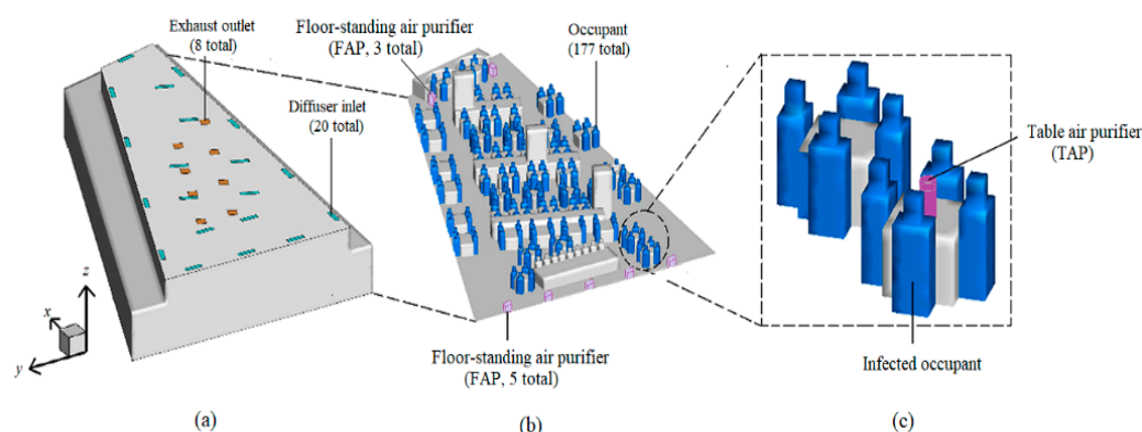
Figure 6. Computer model and components of the restaurant: (a) the placement of exhaust outlets and diffuser inlets; (b) the locations of all occupants; (c) the location of the infected occupant.
