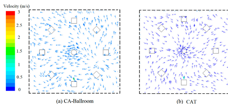
Figure 11. The velocity vector of airflow at the height of the breathing zone ( Z = 1.1\text{ m} ) at the table with the infector under two ventilation conditions.
