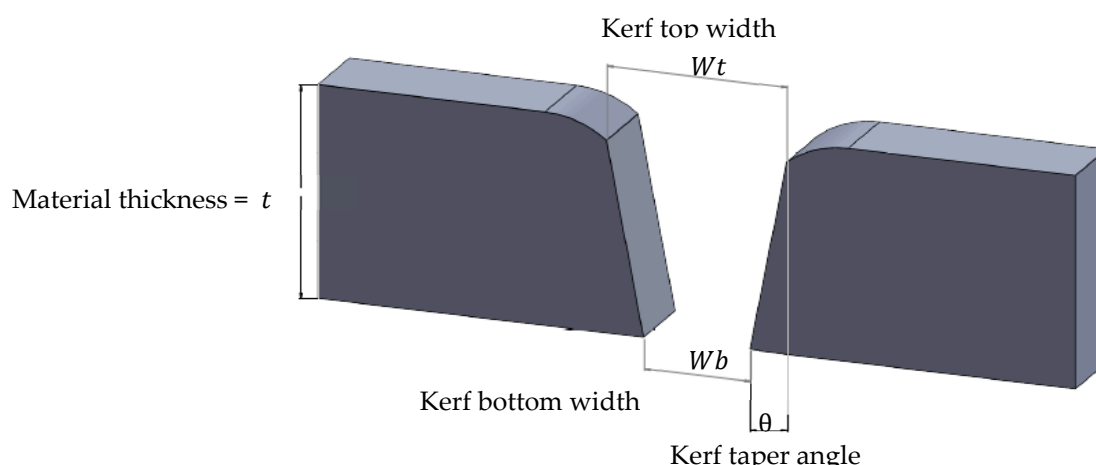
Figure 3. Scheme of AWJM kerf geometries.
