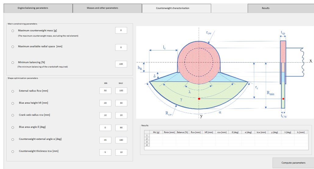
Figure 10. Tab of the user-interface dedicated to the design and optimisation of the counterweights.
