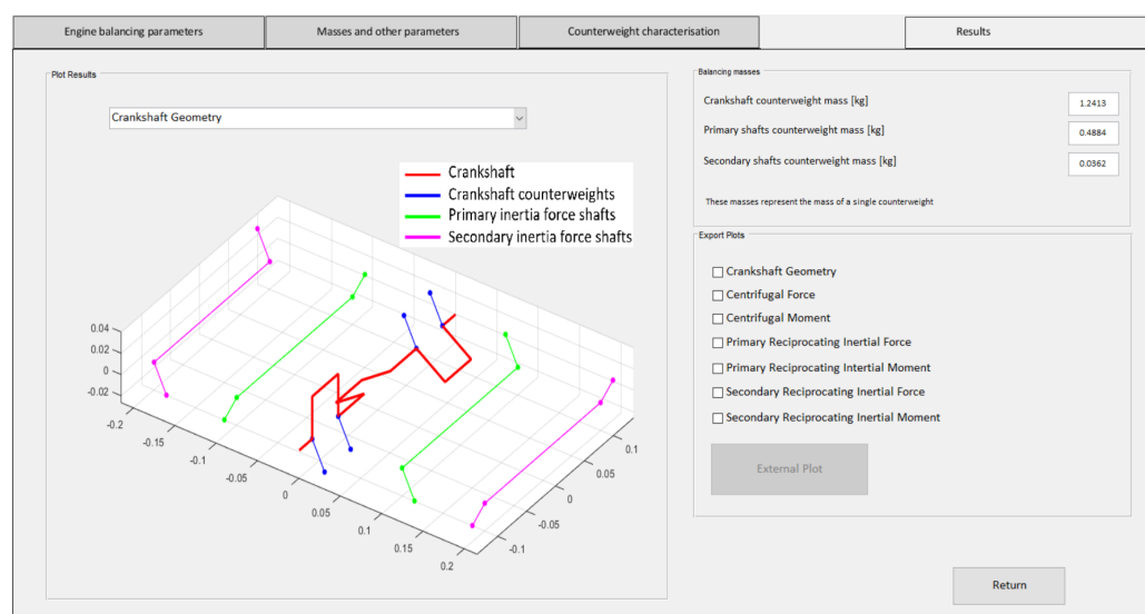
Figure 9. Tab of the user-interface dedicated to the preliminary balancing results.
