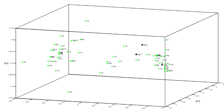
Figure 8. NLPCA scores plot related to finds from Taranto. The fitting parameters with 3 PCs are R^2 = 0.81 and Lof = 0.43. Taranto finds: green triangles Apulian manufacture, green circles traditional manufactures. Black star: a probable firing tester. Black circles: clayey raw materials from a coeval pottery workshop located in Taranto [100,101].
