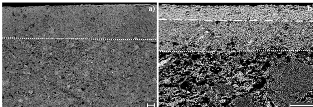
Figure 10. SEM-BSE photomicrographs of thin sections of fragments from Taranto (a) and Monte Sannace (b). The dashed lines separate red engobe layer (upper) from ceramic body (lower), showing the more compact and finer paste of engobe layer with respect to the ceramic body. Scale 100 micron.
