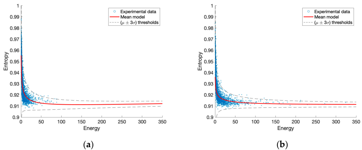
Figure 21. Entropy-energy dispersion, mean model and thresholds for the Colosseum: (a) period from 2011 to 2015; (b) period from 2015 to 2019.
