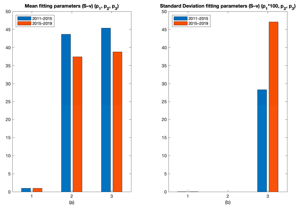
Figure 22. Fitting parameters of the entropy-velocity dispersions in the two periods for the Colosseum: (a) parameters of the mean model; (b) parameters of the standard deviation model.
