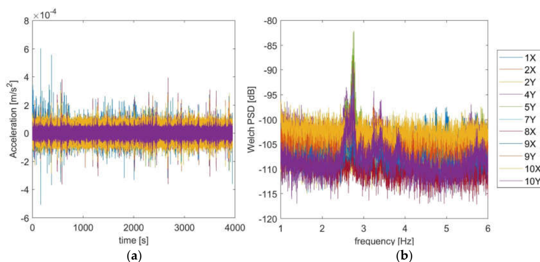
Figure 11. Measured acceleration responses: (a) time-domain; (b) frequency-domain.
