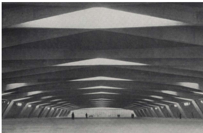
Figure 7. Interior view of Morandi's Pavilion V.
