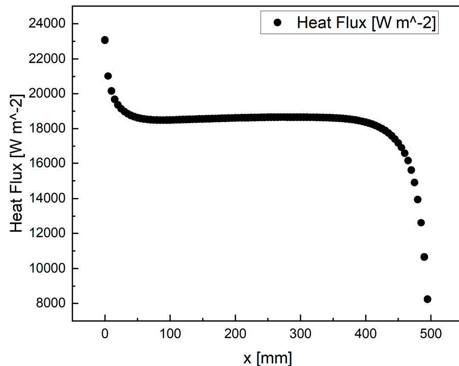
Figure 10. Average heat flux of Tube-3 towards coolant at the heated zone.
