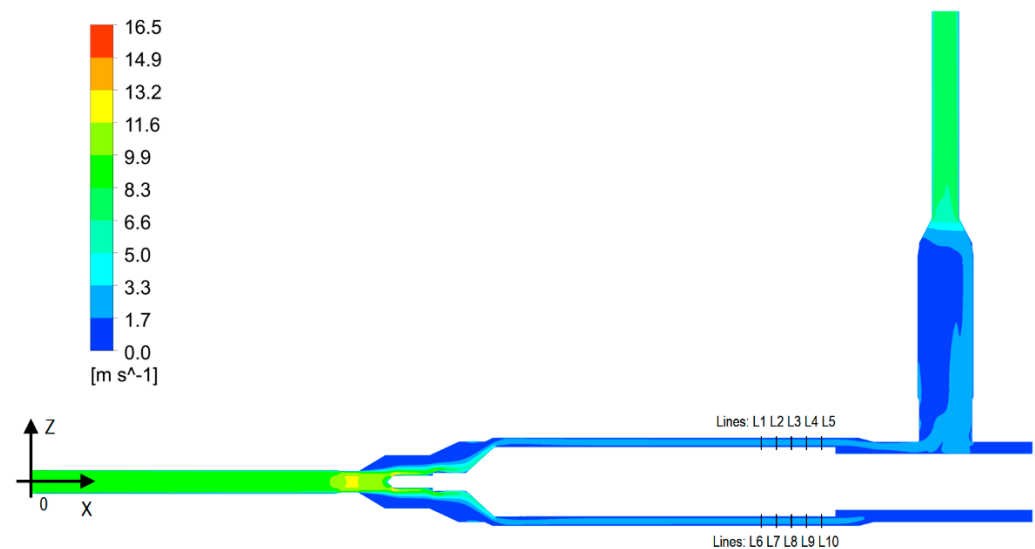
Figure 11. Velocity contour.
