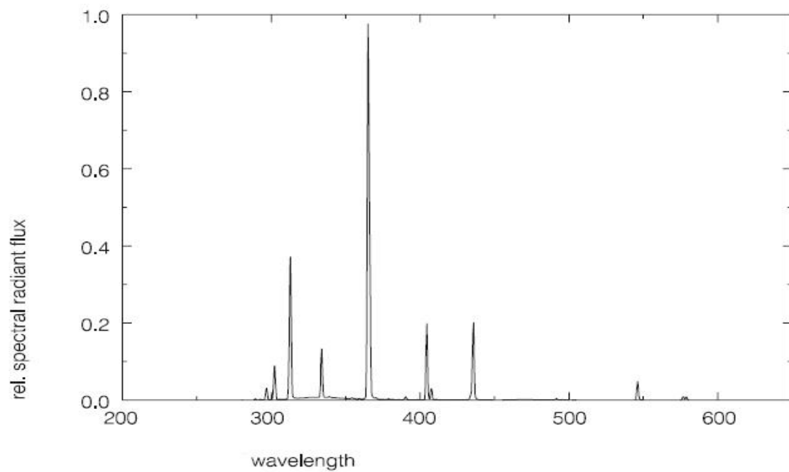
Figure S2. Relative spectral radiant flux of low pressure Hg lamp (TQ 150) being in a glass cooling jacket filled with re-circulated de-ionized water.
