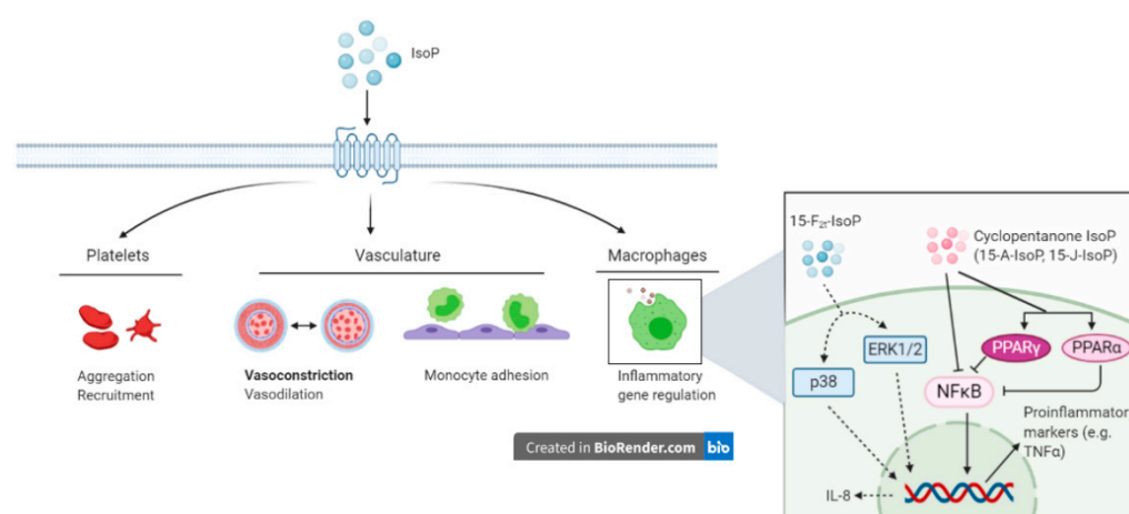
Figure 4. Putative actions of isoprostanes (IsoP) through the thromboxane receptor. Isoprostanes partake in vascular regulation and inflammation through their actions on platelets, the vasculature, and macrophages. During inflammation, IsoP affect monocyte adhesion to the endothelium and alter macrophage inflammatory genes. Insert box: 15-F 2t -isoprostane modifies monocyte adhesion and increases interleukin-8 production via p38 and ERK1/2. Anti-inflammatory effects of IsoP are mediated by signaling through nuclear factor kappa B and peroxisome proliferator-activated receptor. IsoP = isoprostane; ERK = extracellular-signal-regulated kinase; NFκB = nuclear factor kappa B; PPAR = peroxisome proliferator-activated receptor; IL = interleukin. Created with BioRender.com.
