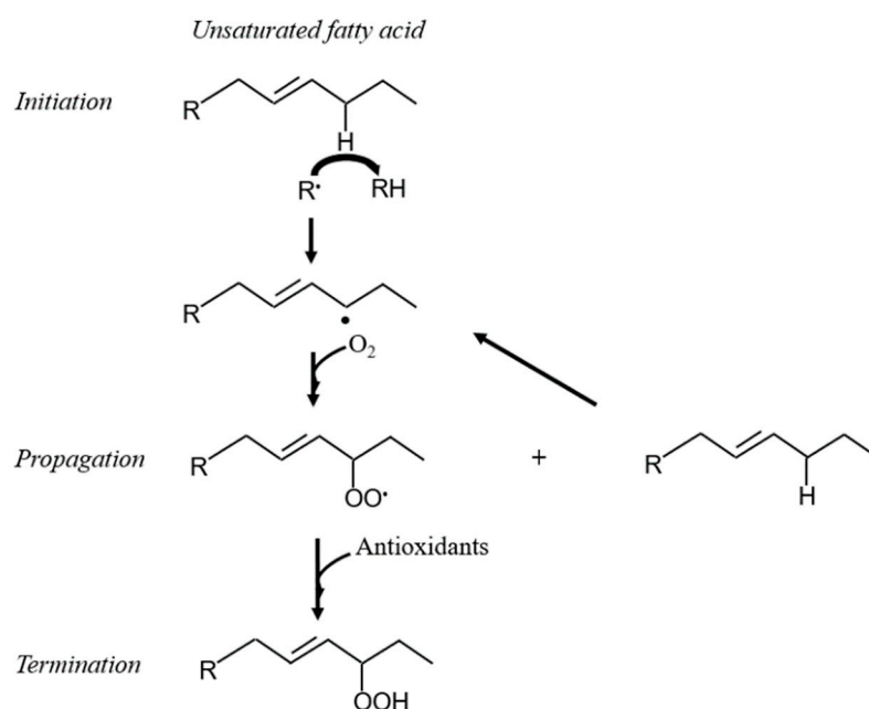
Figure 1. Example of initiation, propagation, and termination pathways during lipid peroxidation. R • = free radical.
