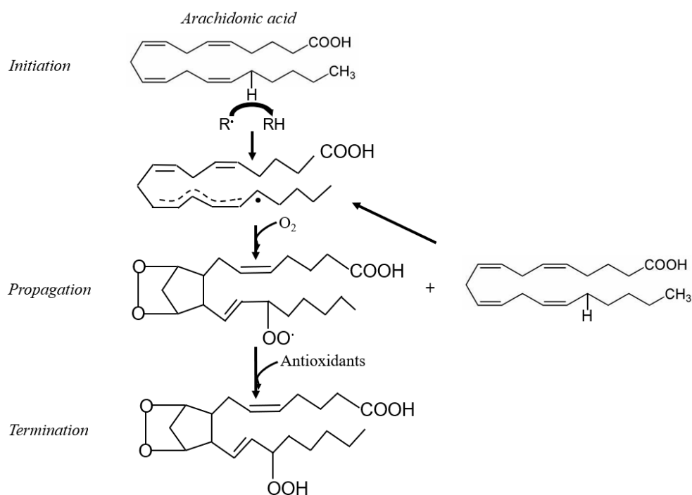
Figure 2. Auto-oxidation of arachidonic acid resulting in the formation of the isoprostane (IsoP) precursor, prostaglandin H (PGH)-like bicyclic endoperoxide. R^\bullet = free radical.
