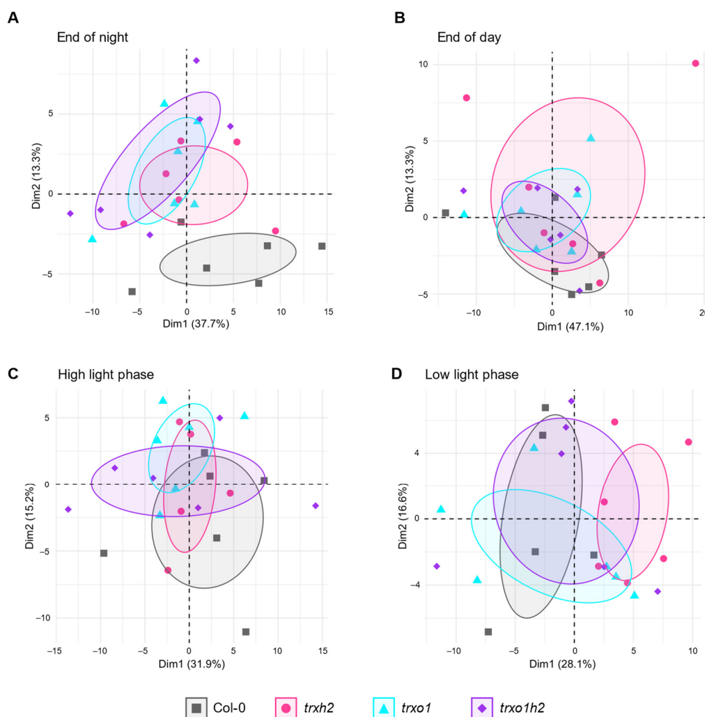
Figure 4. The principal component analysis on metabolite profile of the wild type (Col-0) and the mutant lines ( trxh2 , trxo1 and trxo1h2 ). Arabidopsis plants grown under medium light conditions were harvested at the end of the night (A) and the end of the day (B), respectively. Arabidopsis grown under fluctuating light conditions were harvested at the high-light phase (C) and low-light phase (D), respectively. The samples were used for metabolite profiling via GC-TOF-MS, and the results were used for principal component analysis by using R software. Dim 1: 1st principal component; Dim 2: 2nd principal component.
