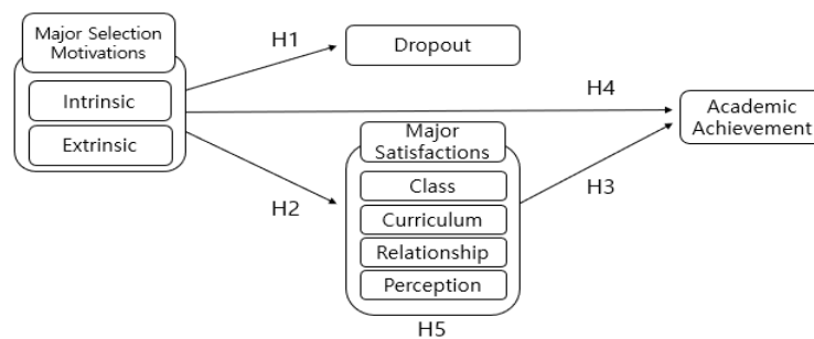
Figure 1. Research Model.
