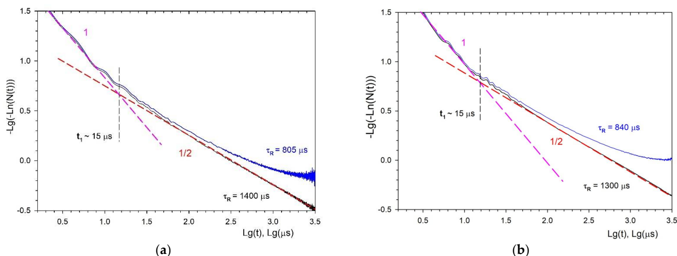
Figure 8. Fluorescence impurity quenching kinetics N(t) = I_{meas}(t) / \exp(-t/\tau_R) (black curves) from the ^4F_{3/2} level of the Nd^{3+} ion in NPs of type I (a) and type II (b) of an aqueous colloidal solution of 0.1 at.% Nd^{3+} : LaF_3 NPs at \tau_R = 1400 \mu s for NPs of type I and at \tau_R = 1300 \mu s for NPs of type II. The blue curve is N(t) when trying to approximate the late stage of luminescence decay kinetics I_{meas}(t) by an exponential function \exp(-t/\tau_R) at (a) \tau_R = 805 \mu s for NPs of type I and (b) at \tau_R = 840 \mu s for NPs of type II. Red dashed lines are Förster kinetics \exp(-0.055\sqrt{t}) and \exp(-0.041\sqrt{t}) . The magenta dashed lines are the ordered decay stage \exp(-W_{ord}t) .
