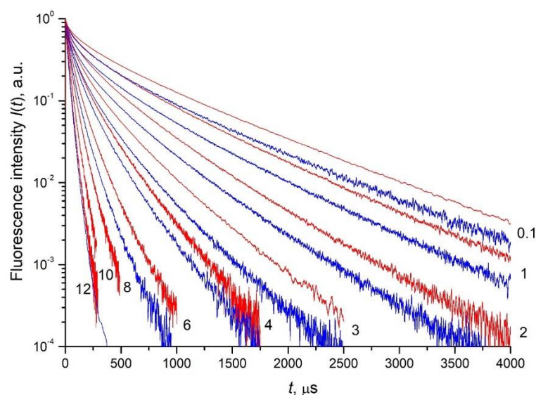
Figure 7. Luminescence decay kinetics of x at% \text{Nd}^{3+} : \text{LaF}_3 ( x is indicated in the figure) detected at the ^4\text{F}_{3/2} \rightarrow ^4\text{I}_{9/2} transition of the \text{Nd}^{3+} ion at \lambda_{\text{det}} = 862.8 nm wavelength upon laser excitation to the ^4\text{G}_{5/2} level ( \lambda_{\text{exc}} = 577.8 nm) for NPs samples of type I (blue curves) and to the ^4\text{F}_{5/2} + ^2\text{H}_{9/2} level ( \lambda_{\text{exc}} = 789 nm) for NPs samples of type II (red curves).
