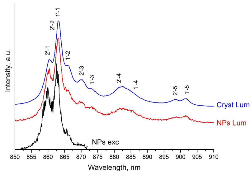
Figure 6. The luminescence excitation spectrum of a 0.1 at% \text{Nd}^{3+}:\text{LaF}_3 NPs sample of type I (black spectrum), measured by scanning a laser at the ^4\text{I}_{9/2} \rightarrow ^4\text{F}_{3/2} transition with a step of 0.12 nm. The detection was performed in the range of 850–873 nm, including ^4\text{F}_{3/2}(j') \rightarrow ^4\text{I}_{9/2}(j) transitions, where j = 1 and 2. The luminescence spectra of a 4 at% \text{Nd}^{3+}:\text{LaF}_3 NPs sample of type I (red spectrum) and 0.45 at% \text{Nd}^{3+}:\text{LaF}_3 single crystal (blue spectrum) upon excitation at a wavelength \lambda_{\text{exc}} = 577.8 nm, measured at the ^4\text{F}_{3/2} \rightarrow ^4\text{I}_{9/2} transition.
