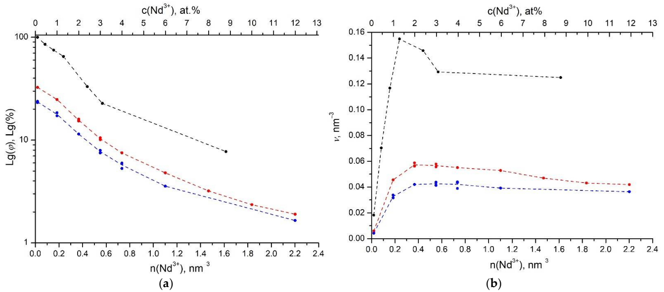
Figure 10. Concentration dependence of the relative quantum yield \varphi (a) and fluorescence brightness \nu (b) of the ^4F_{3/2} level of the \text{Nd}^{3+} ion in single crystals (black circles) and aqueous colloidal solutions of \text{Nd}^{3+} : \text{LaF}_3 NPs samples of type I (blue circles) and type II (red circles) (for NPs samples of type I \tau_R = 1400 \mu\text{s} and NPs of type II \tau_R = 1300 \mu\text{s} ). Dashed blue and red curves are drawn through the arithmetic mean values of the corresponding parameters. For single crystals, the dashed black curve is drawn through the measured values of \varphi and \nu .
