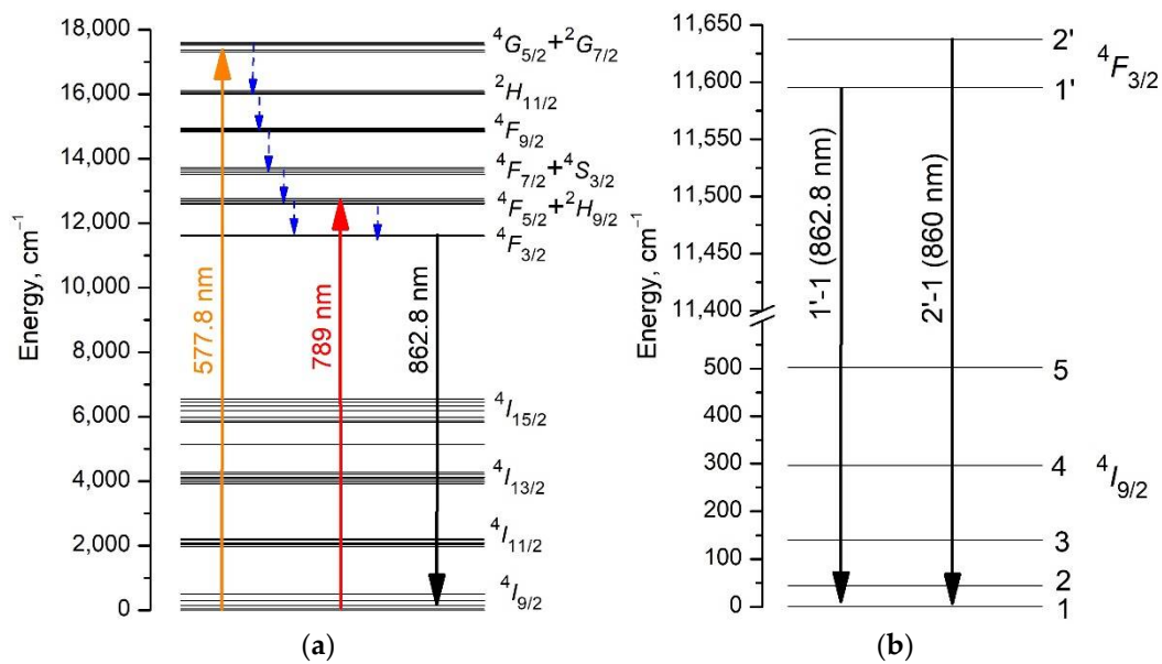
Figure 5. Energy level diagram of the \text{Nd}^{3+} doped \text{LaF}_3 crystal (on the left) [35]: luminescence excitation transitions ^4\text{I}_{9/2} \rightarrow ^4\text{G}_{5/2} + ^2\text{G}_{7/2} (orange arrow) and ^4\text{I}_{9/2} \rightarrow ^4\text{F}_{5/2} + ^2\text{H}_{9/2} (red arrow) and fluorescence transition ^4\text{F}_{3/2} \rightarrow ^4\text{I}_{9/2} (black arrows). Blue dashed arrows indicate multiphonon relaxation of electronic excitations. (a) Crystal field splitting levels (Stark levels) of the ^4\text{I}_{9/2} and ^4\text{F}_{3/2} manifolds of \text{Nd}^{3+} ion in the \text{Nd}^{3+}:\text{LaF}_3 crystal and (b) optical inter-manifold transitions between Stark levels 1'-1 and 2'-1 are shown.
