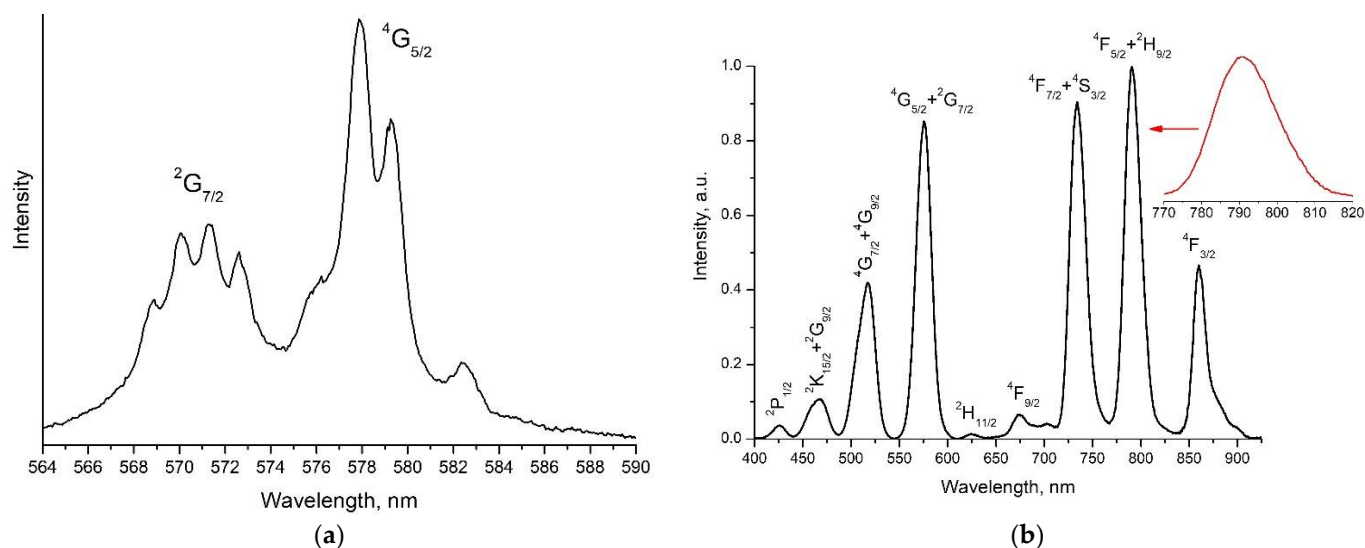
Figure 4. Fluorescence excitation spectrum of the 0.1 at% \text{Nd}^{3+} : \text{LaF}_3 type I NPs sample detected at 862.8 nm when scanning the laser within the ^4\text{I}_{9/2} \rightarrow ^4\text{G}_{5/2} + ^2\text{G}_{7/2} transition wavelengths, normalized to the laser energy (a) and detected at 1064 nm in the range of 400–925 nm (b).
