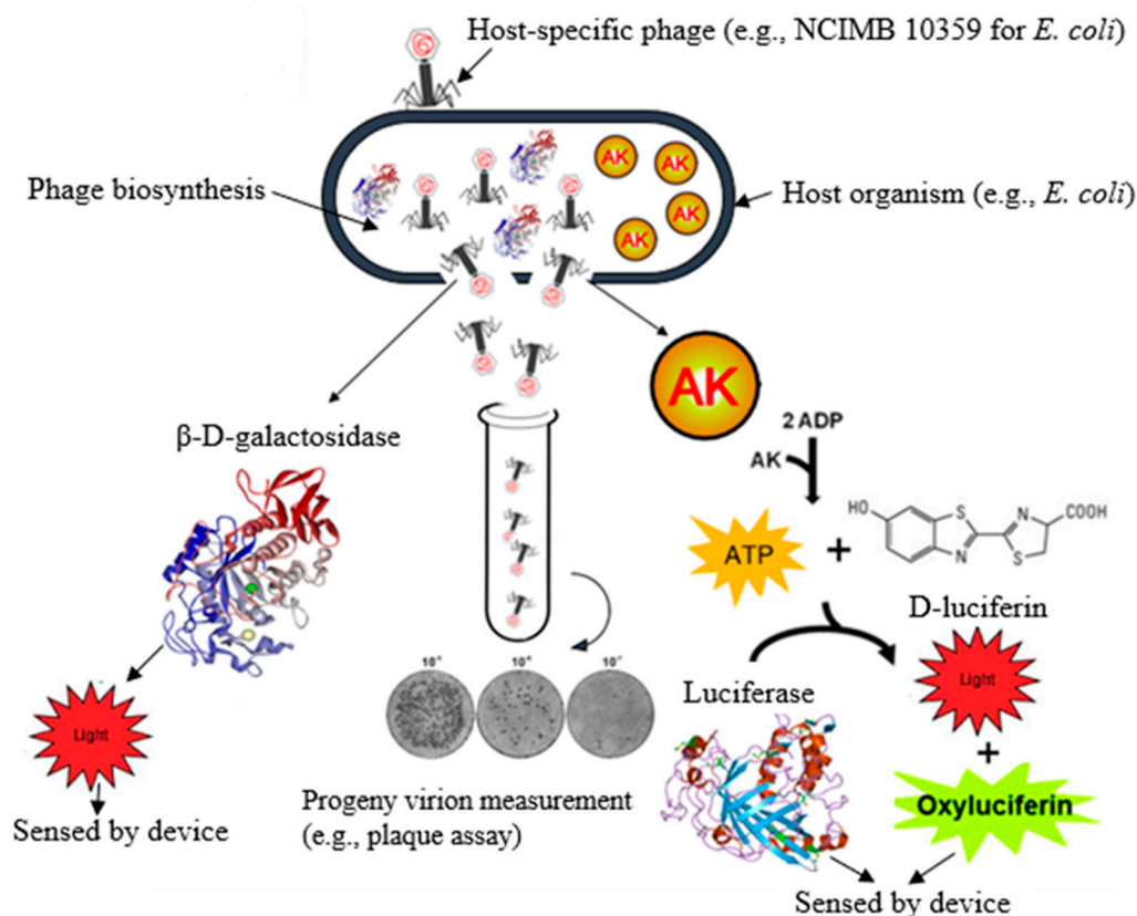
Figure 2. Schematic diagram showing the various intracellular cytoplasmic factors (biomarkers) released following phage infection. Abbr.: AK, adenosine kinase; ATP, adenosine triphosphate.
