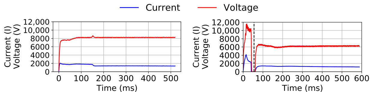
(a) One-phase welding process.
