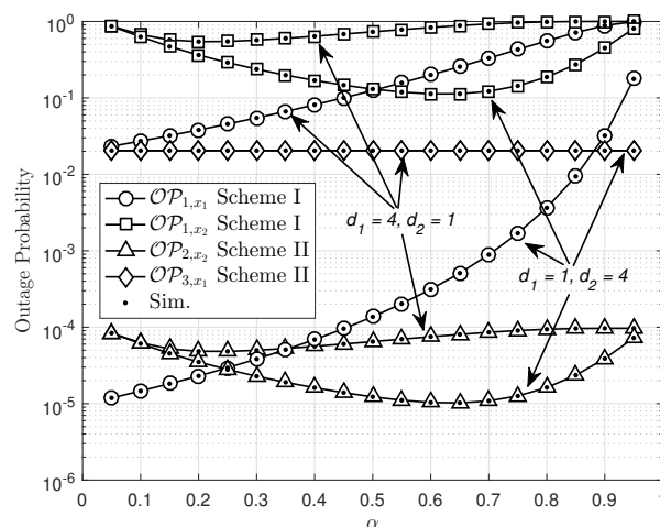
Figure 8. Outage probability versus the power-splitting ratio \alpha with N_S = 2 , N_D = 3 , P_S = 20 dB, a_1 = 0.2 and a_2 = 0.8 .
