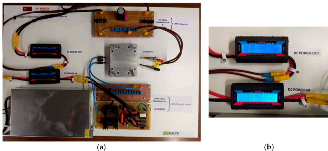
Figure 10. (a) First conceptual prototype of the WPT subsystem of the LiDAR, achieving more than 175 W at 80.5% efficiency. (b) Approximate input and output power readings, using DC power meters.
