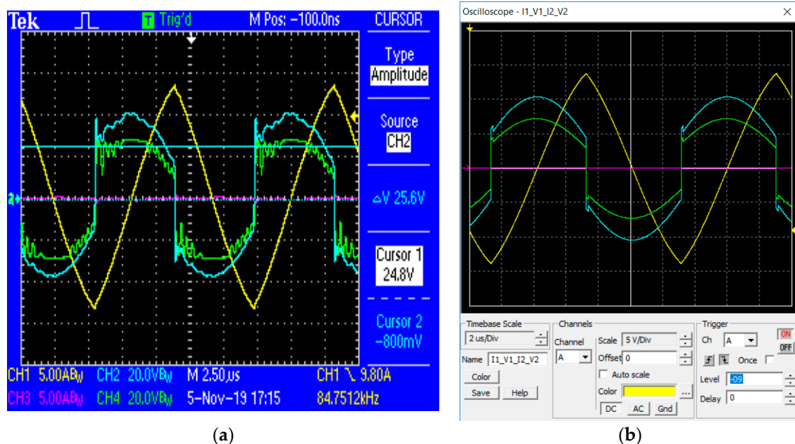
Figure 13. Testing the open secondary load exception: (a) Screen-print of the oscilloscope; (b) Print screen of simulation with PSIM software. Same channels in (a,b), which corresponds to the same signals.
