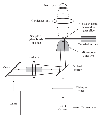
Figure 17. Schematic diagram of the optical tweezers experiment. The laser source is a diode laser operating at \lambda = 532\text{ nm} . The dichroic mirror ensures that most of the laser light reaches the microscope objective. The rail lens is used to vary the size of the laser beam. The objective focuses the laser beam to a spot size of \sim 3\text{ }\mu\text{m} . The sample of polystyrene glass beads in saline solution is placed at the focal spot of the laser. The sample is uniformly illuminated by a backlight. Light from this lamp source passes through a condenser lens and the sample. After passing through the microscope objective, it is imaged on a CCD camera. With the laser blocked, the CCD camera can image the glass beads suspended in solution. When the optical dipole force trap is aligned, the dichroic mirror and dichroic filter ensure that a small fraction of the light scattered by the trapped beads reaches the CCD camera. The scattered light follows the same optical beam path as the backlight and is sufficiently intense for the trapped bead to be imaged.
