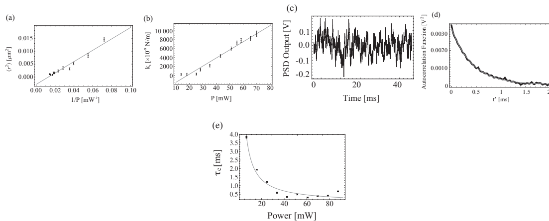
Figure 19. (a) Mean squared displacement as a function of inverse laser power. The power represents the measured value at the entrance to the microscope objective. Only \sim 50\% of the light reaches the sample. (b) Spring constant of the dipole force trap as a function of laser power. The horizontal axis has not been corrected for the power loss at the microscope objective. The points representing the spring constant are calculated from the data in (a) on the basis of the equipartition theorem. (c) Signal from the position sensitive detector (PSD), which represents the position of the bead as a function of time. (d) Autocorrelation function (black) calculated from the PSD signal by fitting to a Lorentzian (grey) for a small section of the data such as in figure (c). The horizontal axis represents the time lag between the data points in the record. The fit gives a correlation time \tau_c = 0.422 \pm 0.005 ms. (e) Correlation time as a function of laser power.
