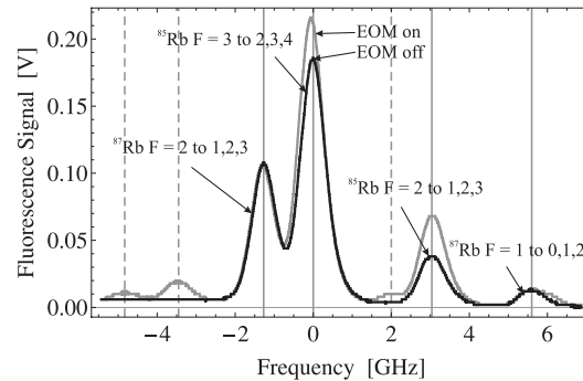
Figure 4. Fluorescence spectra from a pump laser beam passing through an EOM and a Rb vapor cell. The laser is scanned over several GHz and a fluorescence signal is recorded by photodiode C in Figure 3. The black curve shows the fluorescence with the EOM off. The grey curve is obtained with the EOM on. The operating frequency of the EOM is 2.915 GHz which represents the energy difference between the F = 3 \rightarrow F' = 4 and F = 2 \rightarrow F' = 3 transitions in ^{85}\text{Rb} .
