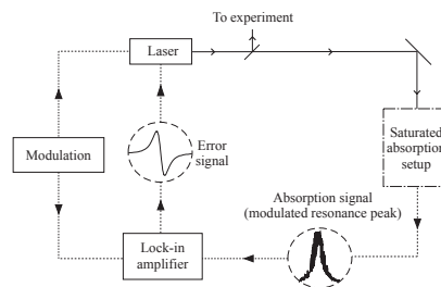
Figure 8. Setup for laser frequency stabilization using a lock-in amplifier. The modulation was provided by a function generator operating at \sim 7 kHz. A scan controller is used to scan the laser frequency at a rate of \sim 10 Hz. An example of the saturated absorption signal obtained by scanning the laser over a single Doppler-free transition is shown. For illustrative purposes, this trace was recorded with a large amplitude for frequency modulation. The output of the lock-in amplifier generates the corresponding dispersion shaped error signal. To lock the laser to the peak of this resonance line, the laser frequency is centered on the resonance peak, and the scan amplitude is gradually reduced (ideally to zero) before engaging the feedback loop.
