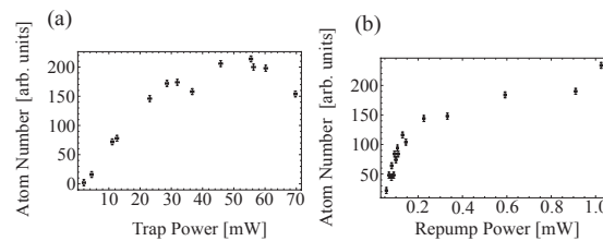
Figure 22. (a) Steady state atom number as a function of trap laser power. The atom number is inferred by recording the trap fluorescence on a photodiode. The voltage recorded by the detector can be converted into atom number. The maximum voltage corresponds to an atom number of \sim 10^7 . Since the trap laser is retro-reflected through the vacuum chamber, the laser power incident on the atoms is approximately twice the trap laser power. (b) Atom number as a function of repump laser power. For both of these experiments, the trap laser detuning was fixed at 15 MHz below resonance, the trapping beam diameter was \sim 0.90 \text{ cm} and the magnetic field gradient was \sim 7 \text{ G/cm} .
