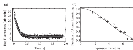
Figure 27. (a) Measurement of the optical molasses decay time. A fit to a decaying exponential gives a 1/e time constant of 0.165 \pm 0.002 s. (b) Measurement of the temperature of trapped atoms using the release and re-capture method. The vertical axis represents the fraction of re-captured atoms. The horizontal axis is the free expansion time. A determination of the most probable speed u from the fit gives a temperature T = 420 \pm 20 \mu K.
