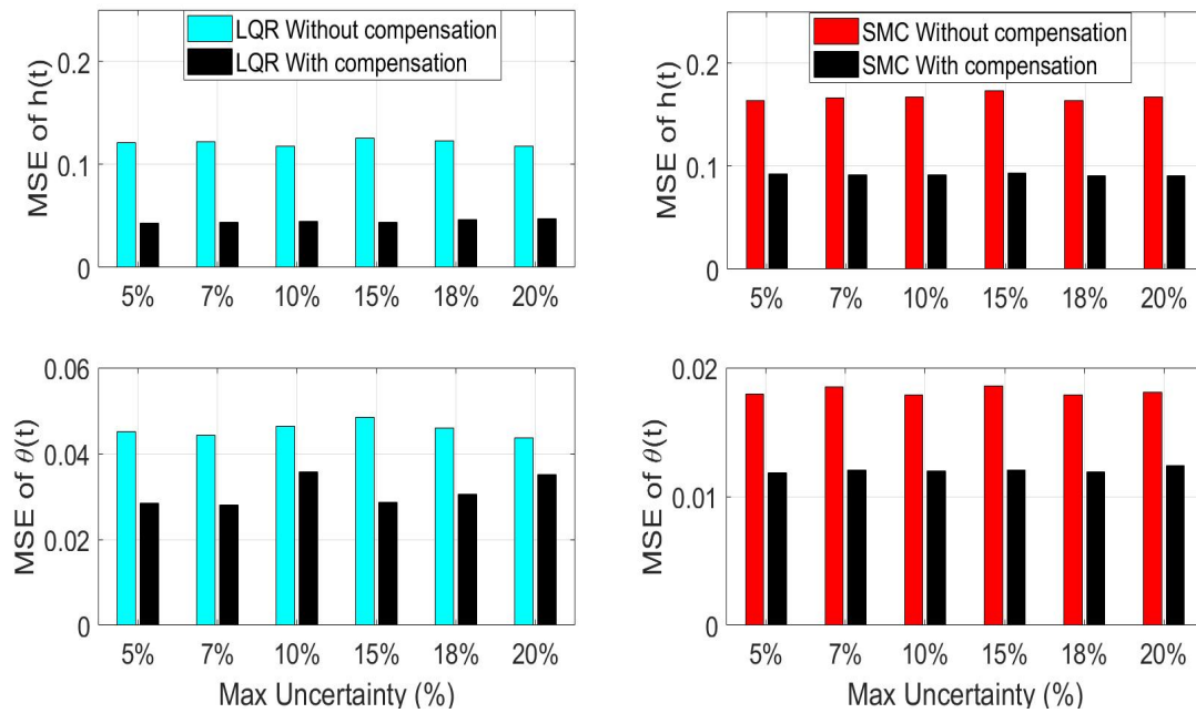
Figure 5. Average mean squared error (MSE) during closed-loop operation for 10 iterations of randomized parameter uncertainty using LQR ( left ) and SMC ( right ) with and without uncertainty compensation.
