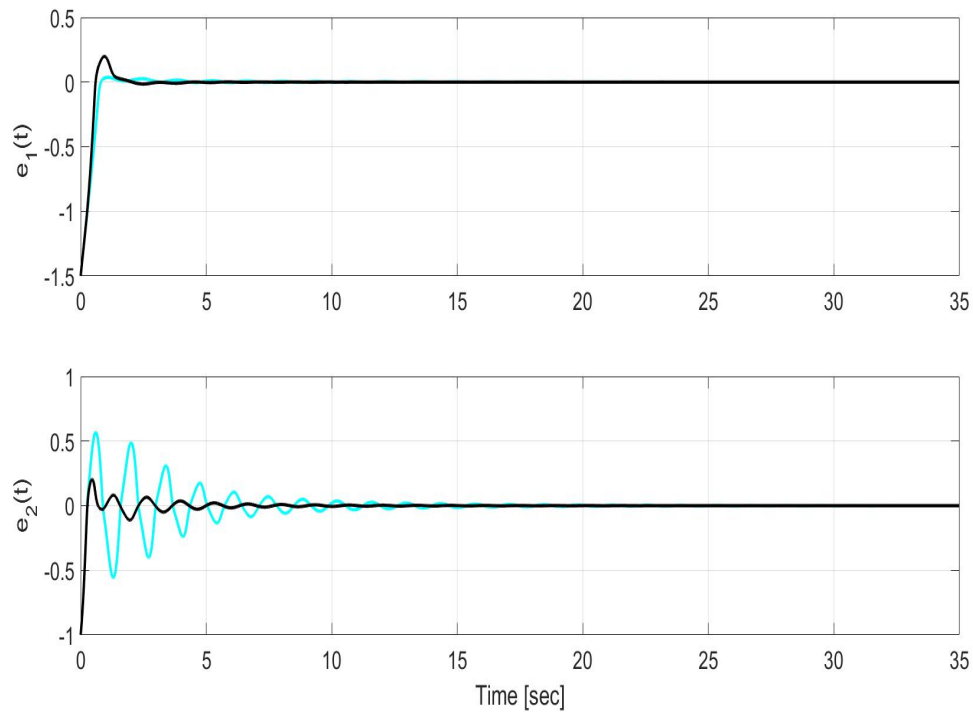
Figure 6. Time evolution of the estimation error in states h(t) ( top ) and \theta(t) ( bottom ) for LQR without uncertainty compensation (cyan) and LQR with uncertainty compensation (black) over the entire simulation time.
