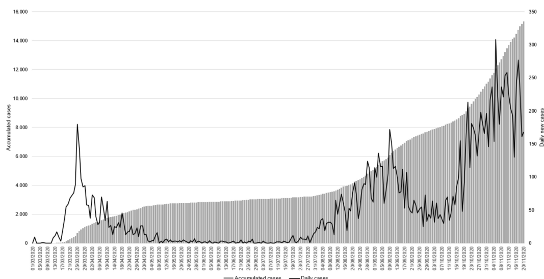
Figure 2. Daily and cumulative trend in COVID-19 cases in the Community of Cantabria (first method stage: March–November 2020). Scheme 19 [29], in Cantabria (open data from the Government of Cantabria).
