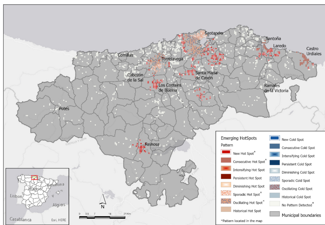
Figure 5. Emerging hotspots for COVID-19 in the Autonomous Community of Cantabria (March–November 2020). Scheme 22 [29]. Source: Own work based on COVID-19 microdata daily records from the health authorities (Government of Cantabria, Spain).
