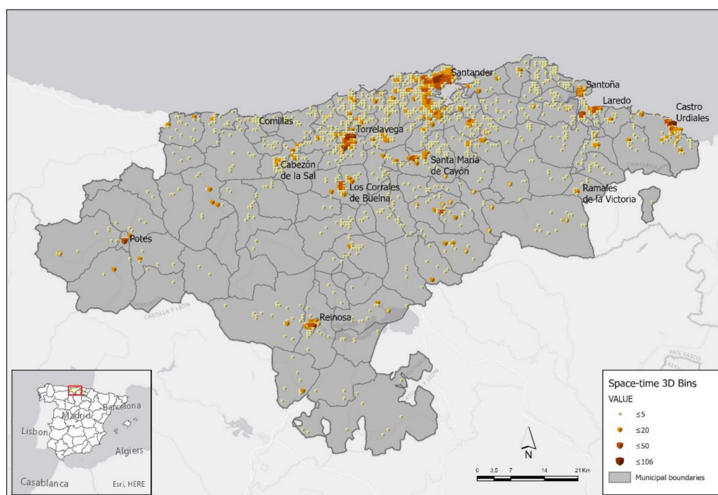
Figure 4. Space–time 3D bins of COVID-19 in the Autonomous Community of Cantabria (March–November 2020). Source: Own work based on COVID-19 microdata daily records from the health authorities (Government of Cantabria, Spain).
