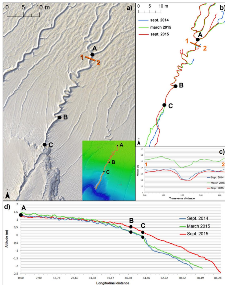
Figure 9. (a) Display of a micro-creek in the inter-tidal zone on an extract of the orthophoto of March 2015 (and in the inset, the corresponding position on an extract of the DEM); (b) diachronic monitoring of the micro-creek position. The thalweg of the micro-creek is manually plotted from the orthophotographs using ArcGIS® software. (c) Example of a transverse profile showing the incision shape and the depth of the micro-creek; (d) example of a longitudinal profile.
