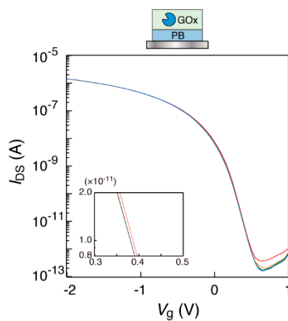
Figure S1. Transfer characteristic curves of the organic field-effect transistor (OFET) biosensor with a GOx-PB electrode in a buffer solution (1× PBS) at 25°C. Scan times = 4. The inset shows the enlarged view.
