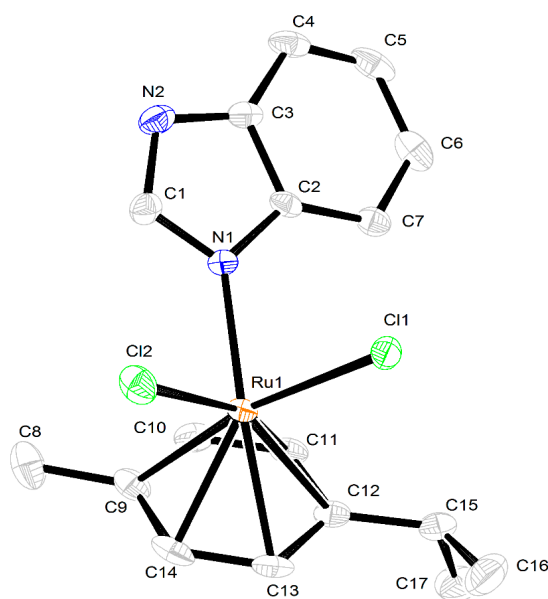
Figure 5. X-ray molecular structure of complex 3 . Thermal ellipsoids are drawn at a 50% probability level. Hydrogen atoms are omitted for clarity.
