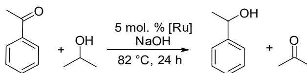
Scheme 4. Transfer hydrogenation of acetophenone catalyzed by complexes 1–3.
