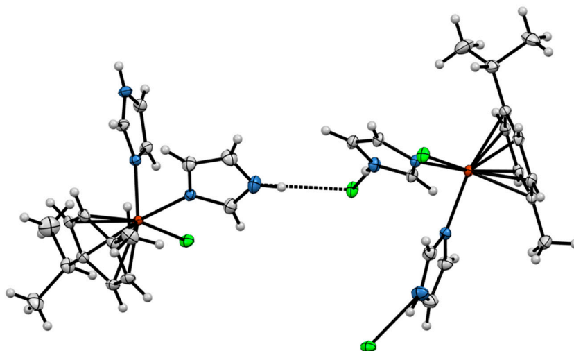
Figure 3. Intermolecular N–H⋯Cl interactions in the crystal structure of complex 1 .
