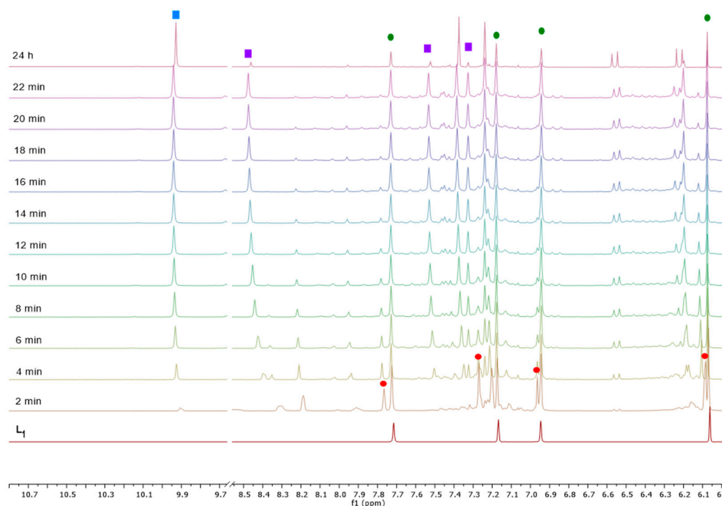
Figure 1. NMR 1 H (500 MHz) monitoring of the reaction between [Ru( p -cym)Cl 2 ] 2 and L1 in MeCN- d_3 . Signal assignments: L1 —red circles; Ru- L1 intermediate complex—green circles; Ru-imidazole complex—purple squares; formaldehyde—blue square.
