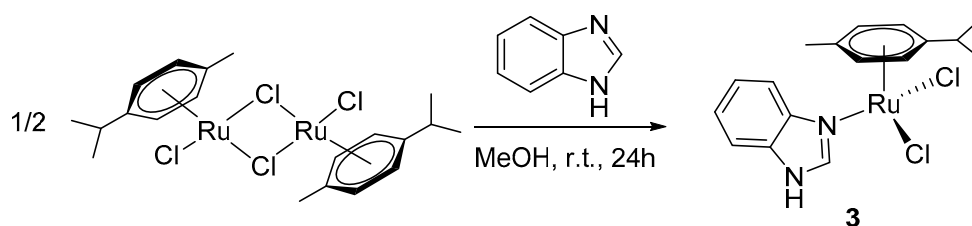
Scheme 3. Synthesis of complex [\text{Ru}(\text{BImH})(p\text{-cym})\text{Cl}_2] ( 3 ).
