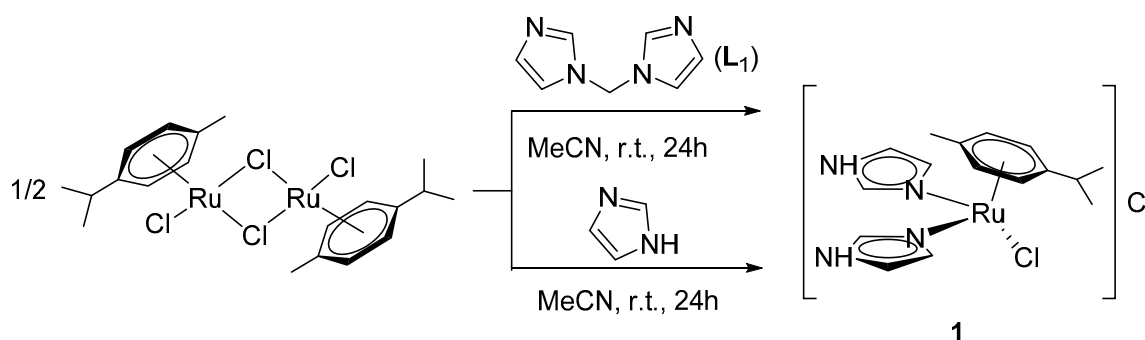
Scheme 1. Synthesis of complex [\text{Ru}(\text{ImH})_2(p\text{-cym})\text{Cl}]\text{Cl} ( 1 ).
