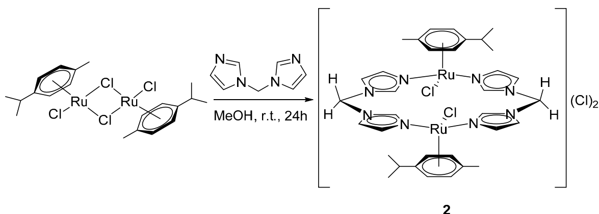
Scheme 2. Synthesis of complex [\text{Ru}_2(\text{L}1)_2(p\text{-cym})_2\text{Cl}_2]\text{Cl}_2 ( 2 ).
