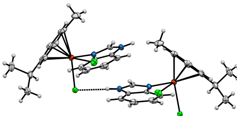
Figure 6. Intermolecular N–H···Cl interactions in the crystal structure of complex 3.
