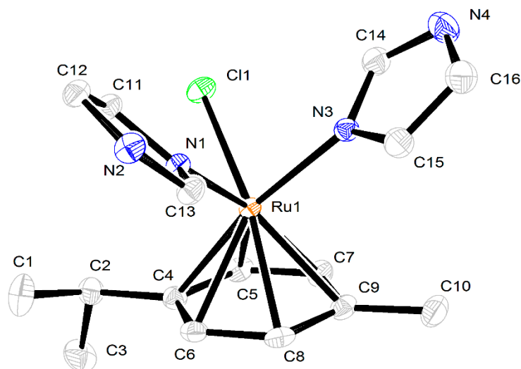
Figure 2. X-ray molecular structure of complex 1 . Thermal ellipsoids are drawn at a 50% probability level. Hydrogen atoms and Cl − anions are omitted for clarity.
