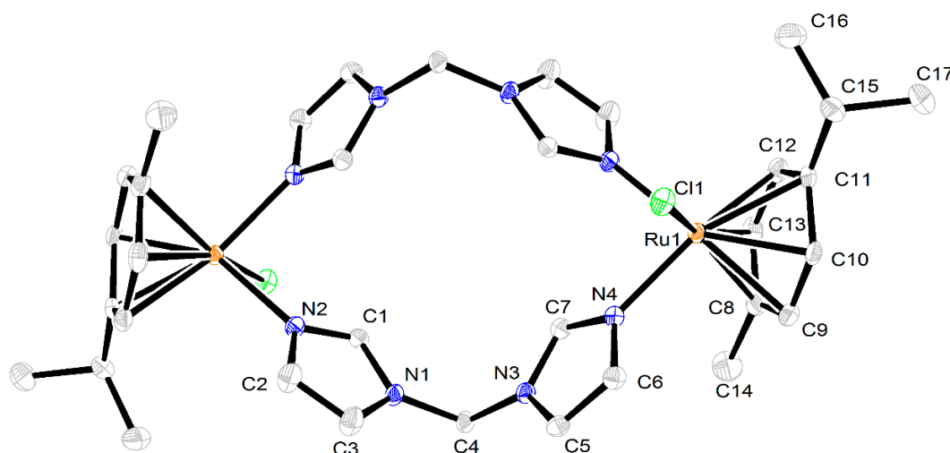
Figure 4. X-ray molecular structure of complex 2 . Thermal ellipsoids are drawn at a 50% probability level. Hydrogen atoms, solvate methanol molecules, and Cl − anions are omitted for clarity.
