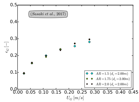
Figure 19. Influence of AR in large diameter bubble columns with spider sparger—data from ref. [28].
