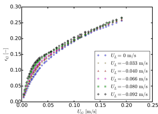
Figure 16. Pipe sparger in open tube configuration—data from ref. [34].
