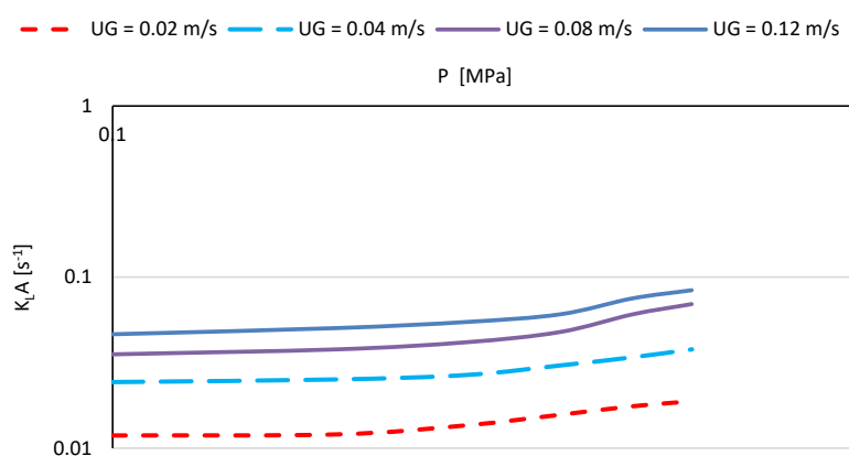
Figure 34. Influence of the operating pressure on k_{LA} —data from Kang et al. [179]—even distribution experimental data.
