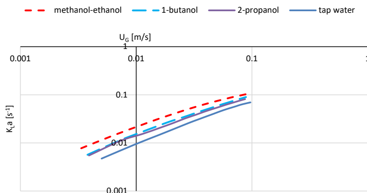
Figure 37. Influence of the gas phase on k_{La} —data from Ozturk et al. [173].
