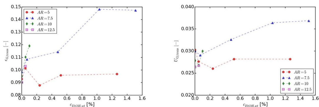
(a) Influence of AR and the concentration ( c ) on the transitional gas hold-up
