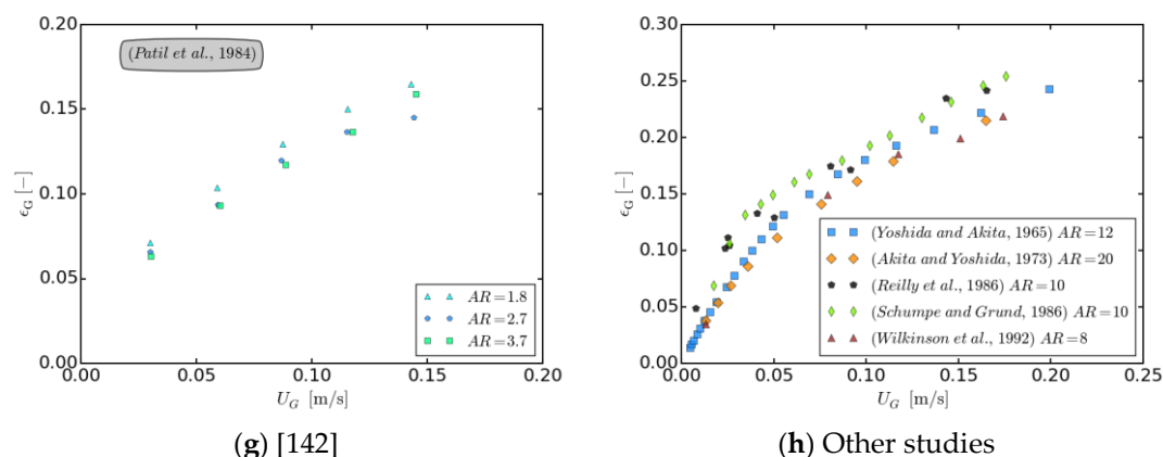
Figure 20. Influence of the aspect ratio in large diameter bubble columns—studies from the literature.
