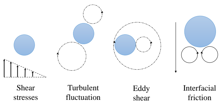
Figure 41. Break-up mechanisms.
