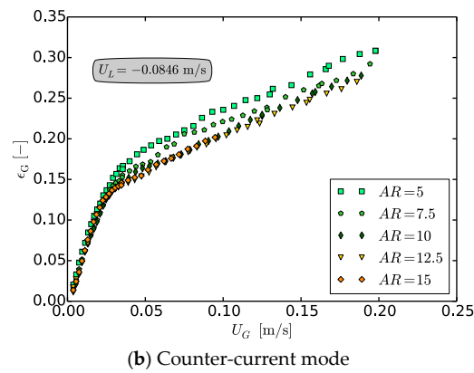
Figure 19. Influence of AR in large diameter bubble columns with spider sparger—data from ref. [28].
