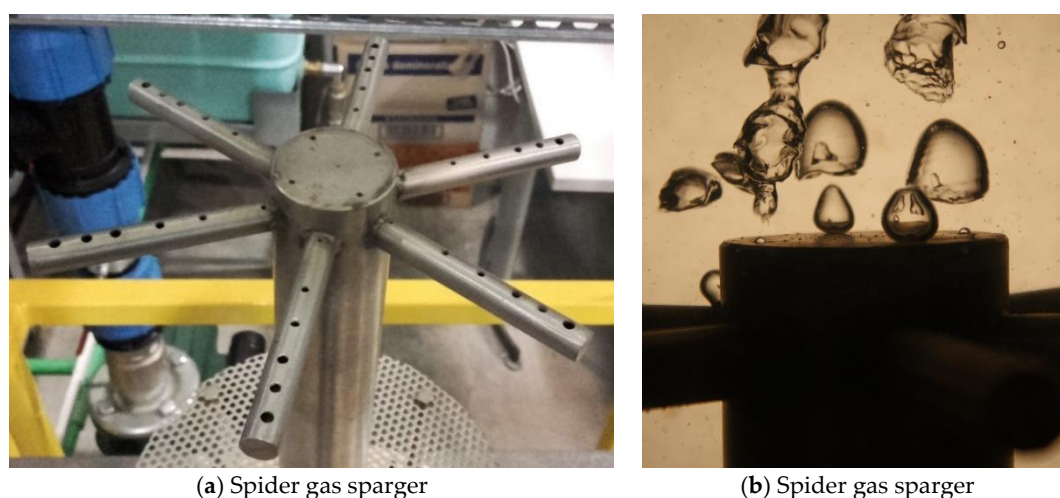
Figure 6. “Coarse gas sparger”.
