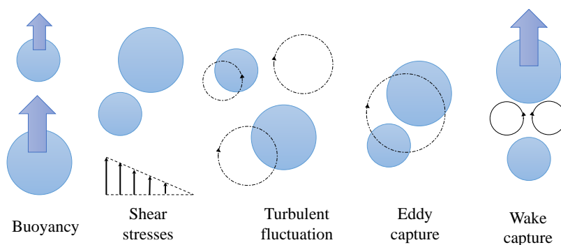
Figure 40. Coalescence mechanisms.
