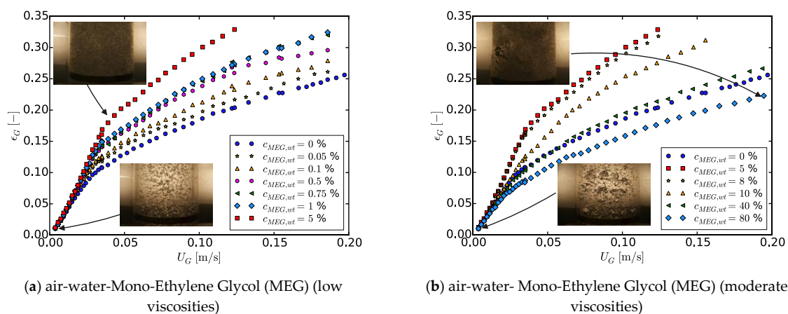
Figure 22. Flow regime maps.
