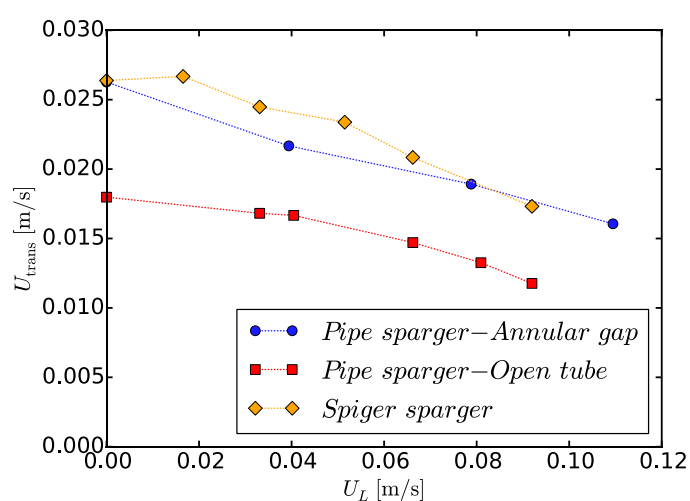
(b) Influence of U_L on the transitional gas velocity
