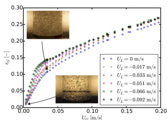
Figure 18. Spider sparger—data from ref. [46].
