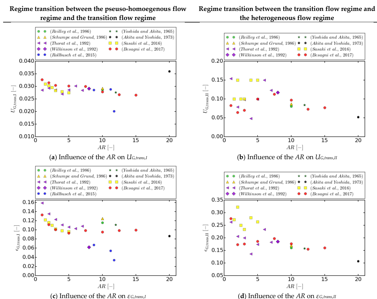
Figure 4. Influence of the aspect ratio (AR) on flow regime transition points—data obtained by [28].
