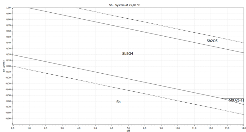
Figure S9. Eh-pH diagram of Sb.
