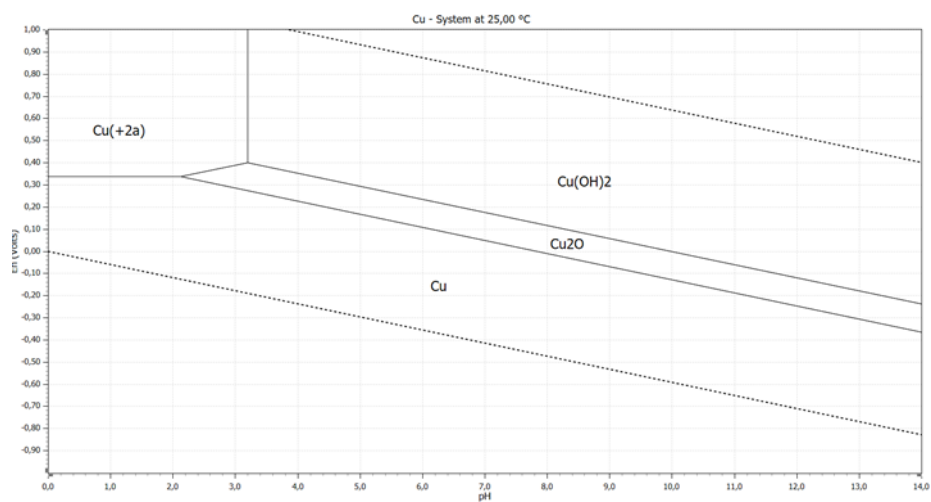
Figure S2. Eh-pH diagram of Cu.
