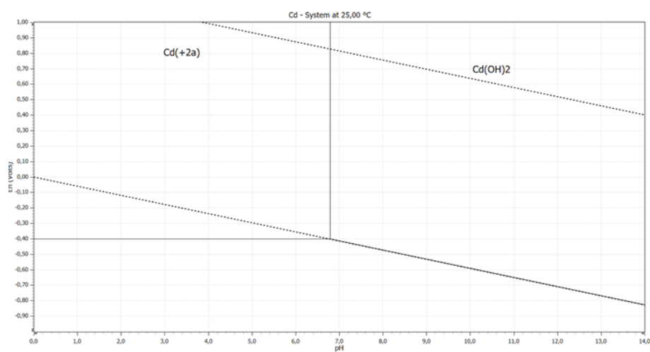
Figure S8. Eh-pH diagram of Cd.
