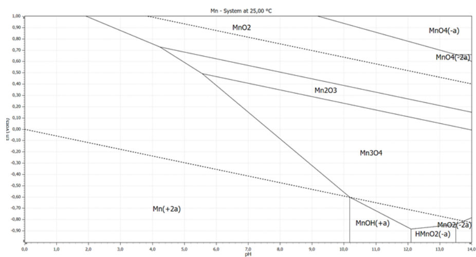
Figure S5. Eh-pH diagram of Mn
