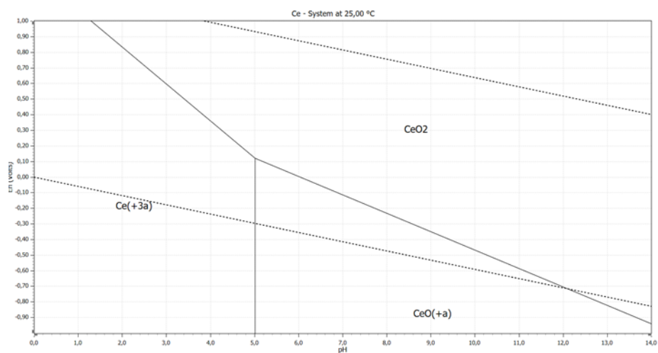
Figure S10. Eh-pH diagram of Ce.
