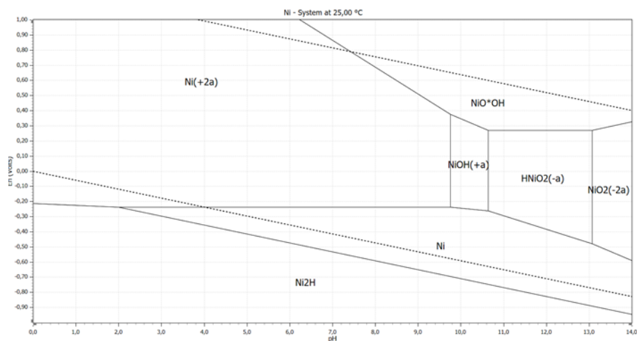
Figure S15. Eh-pH diagram of Ni.
