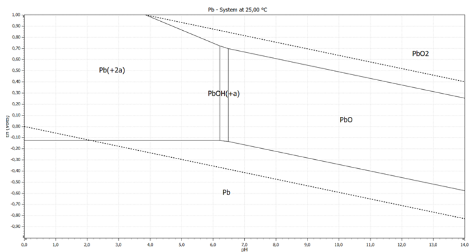
Figure S13. Eh-pH diagram of Pb.
