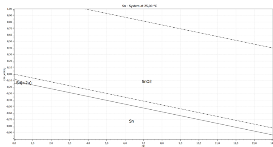
Figure S12. Eh-pH diagram of Sn.
