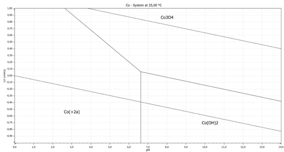
Figure S1. Eh-pH diagram of Co.
