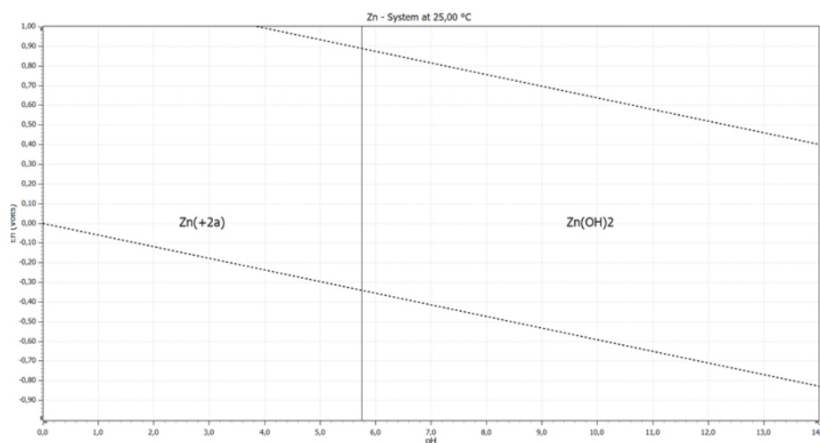
Figure S7. Eh-pH diagram of Zn.
