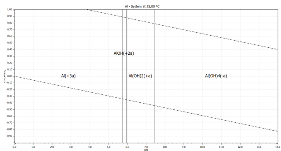
Figure S14. Eh-pH diagram of Al.
