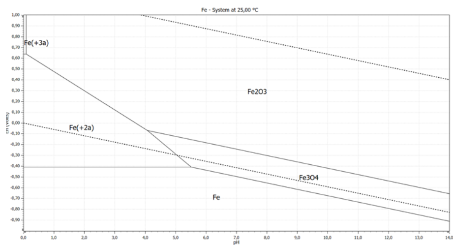
Figure S3. Eh-pH diagram of Fe.
