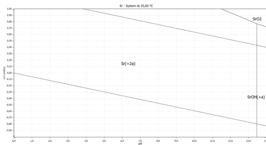
Figure S6. Eh-pH diagram of Sr.
