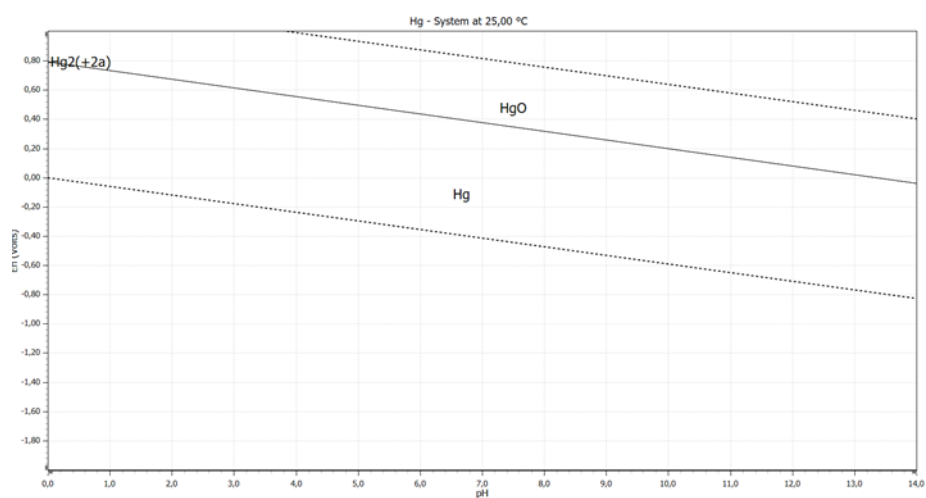
Figure S11. Eh-pH diagram of Hg.
