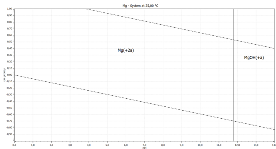
Figure S4. Eh-pH diagram of Mg
