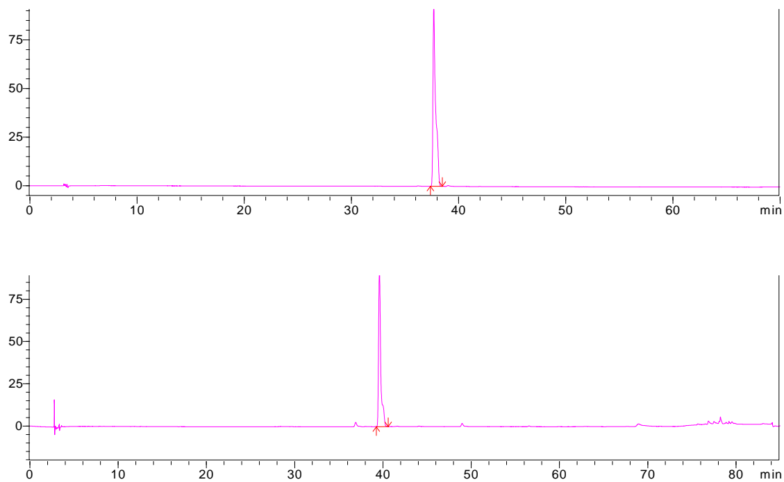
Figure S1: Chromatograms recorded as 280 nm, of narirutin (upper figure) and hesperidin (lower figure) standards. Both compounds were dissolved in HPLC-grade methanol at 50 \mu\text{g mL}^{-1} .
