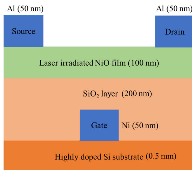
Figure 1. Layered structure of laser-irradiated \text{NiO}_x -based TFT (Staggered bottom gate TFT).
