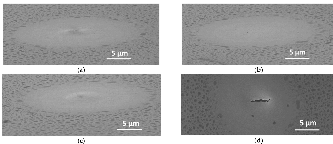
Figure 2. Scanning Electron Microscope images of laser-irradiated \text{NiO}_x/\text{SiO}_2 TFT (Scale: 1 inch = 10 \mu\text{m} ). (a) Laser fluence of 125 \text{ mJ/cm}^2 , (b) 150 \text{ mJ/cm}^2 , (c) 175 \text{ mJ/cm}^2 and (d) 200 \text{ mJ/cm}^2 .
