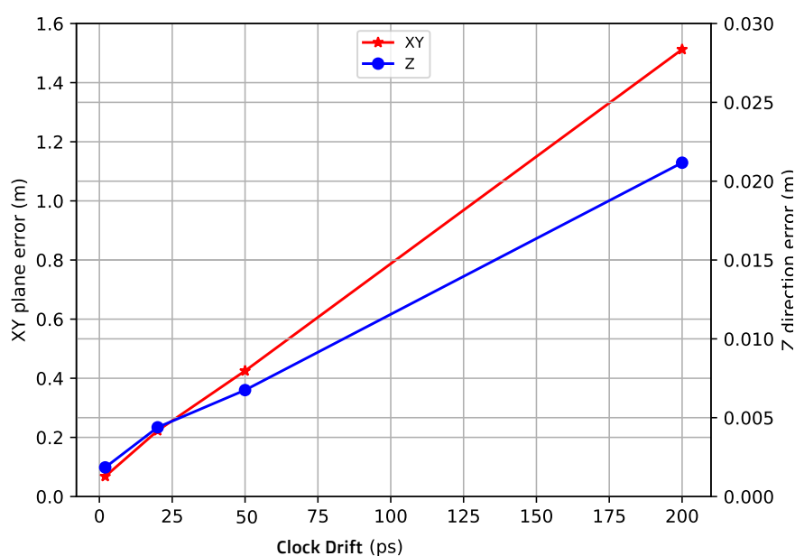
Figure 4. Localization error with respect to clock drifts.
