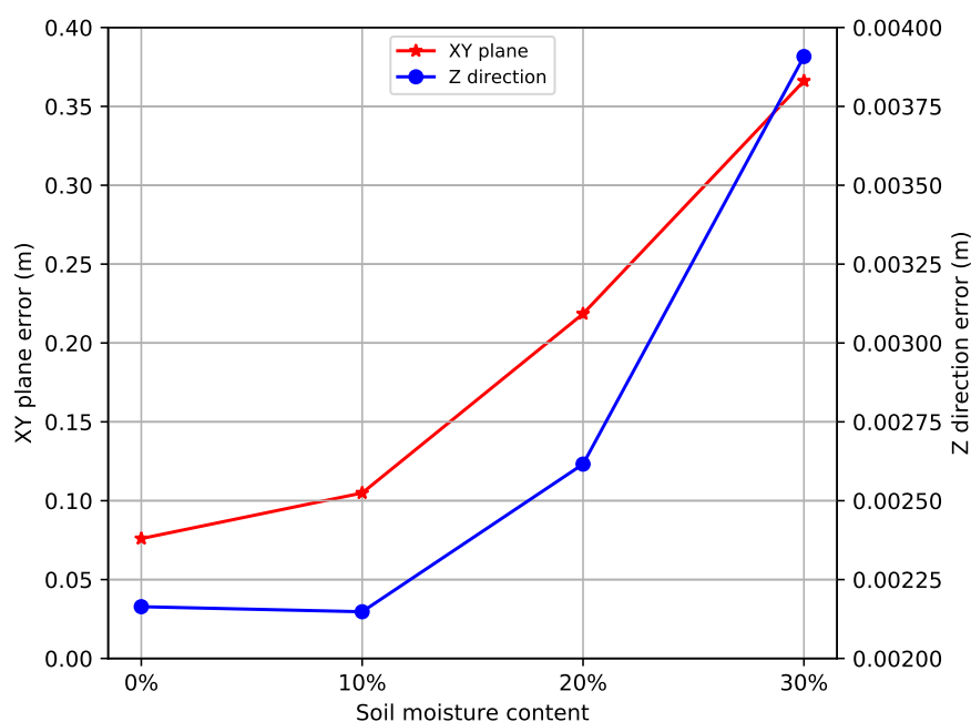
Figure 3. Localization error with respect to moisture content.
