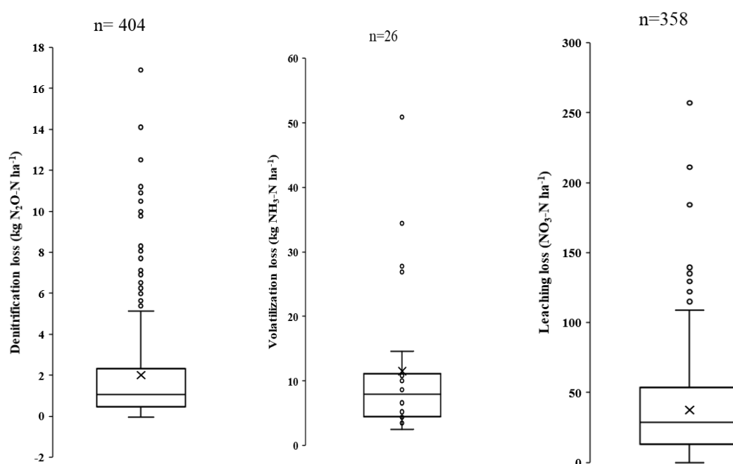
Figure 1. Extent of cumulative nitrogen losses ( \text{kg N ha}^{-1} ) during growing season from non-leguminous field crops, generated from data published in peer-reviewed manuscripts.
