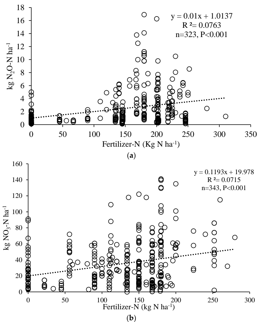
Figure 2. Linear regression relationship between fertilizer N application rate (kg N ha -1 ) and (a) cumulative nitrous oxide flux (kg N 2 O-N ha -1 ) and (b) leaching loss of nitrate (kg NO 3 -N ha -1 ) within corn production system.
