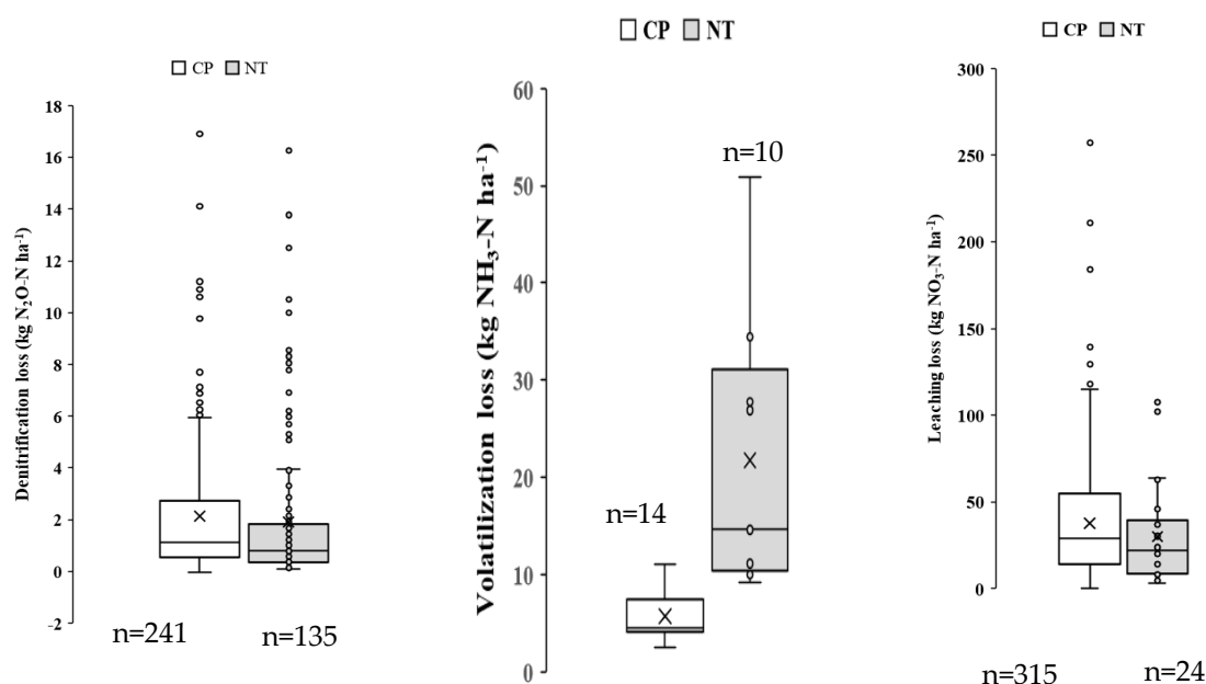
Figure 3. Nitrogen losses ( \text{kg N ha}^{-1} ) as influenced by chisel (CP) and no-tillage (NT) practices.
