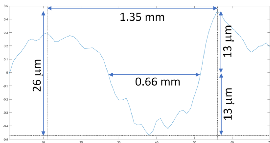
Figure 9. Profilometry of the scratch on the surface of the digging stick replica, obtained from the 3D model of the surface shown in Figure 8.
