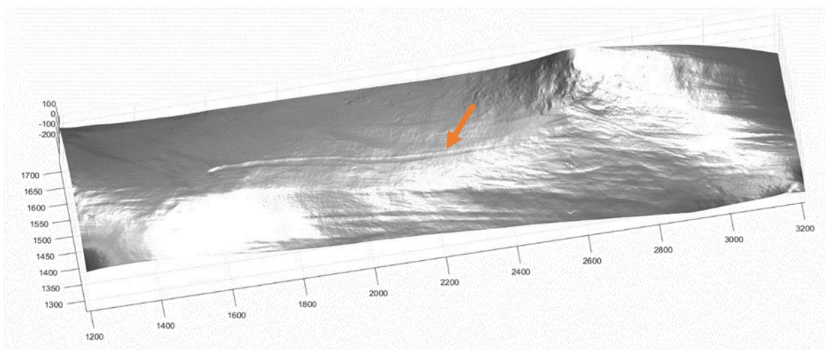
Figure 8. 3D reconstruction of the wood surface. The red arrow identifies the point where the surface scratch depth profile was reconstructed.
