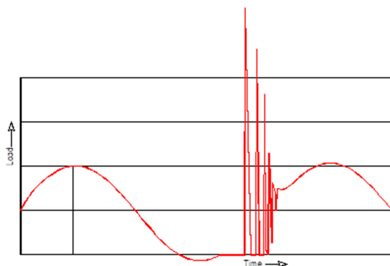
Figure 9. Slack towline followed by a large peak load ( \approx 2.5 \times \text{Amplitude} ) [17]. Drawing: Authors.
