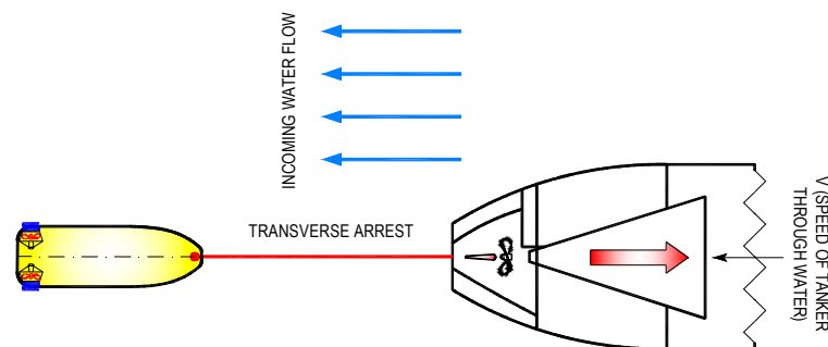
Figure 5. Transverse arrest mode by an ASD escort tug (6–8 knots). A transitional mode between direct and indirect methods. Drawing: Authors.
