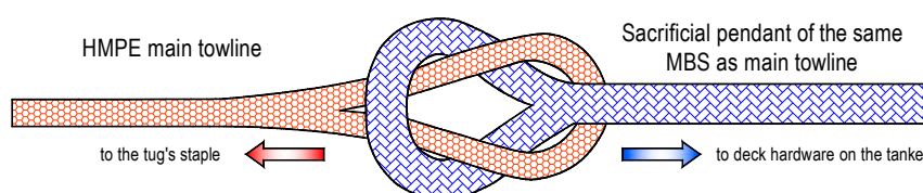
Figure 14. Cow hitch connecting HMPE towline to a sacrificial pendant. Drawing: Authors.
