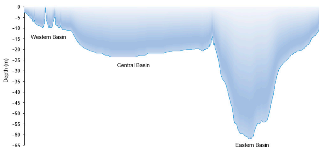
Figure 4. Lake Erie depth profile in meters from west to east.
