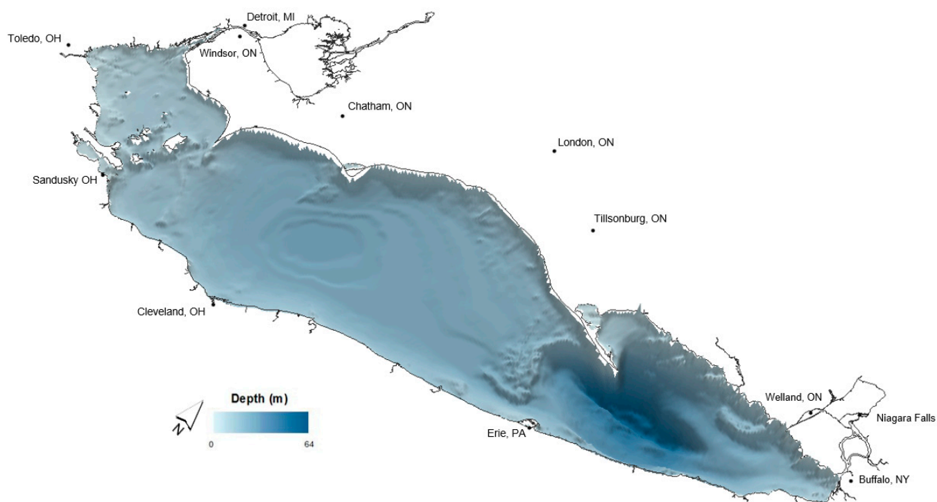
Figure 6. Bathymetry of Lake Erie from the southeast perspective.
