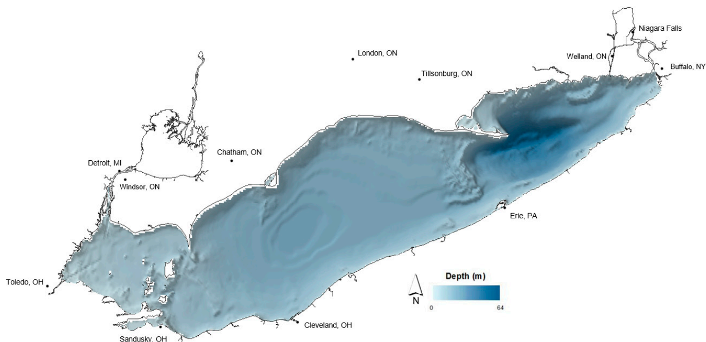
Figure 5. Bathymetry of Lake Erie viewed from the normal southern position.
