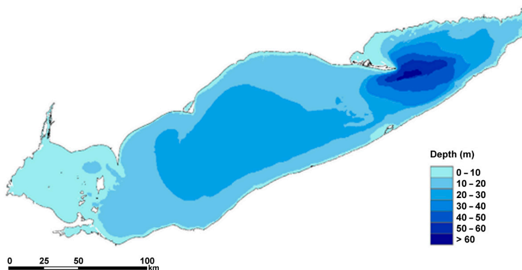
Figure 2. Lake Erie depth (m).
