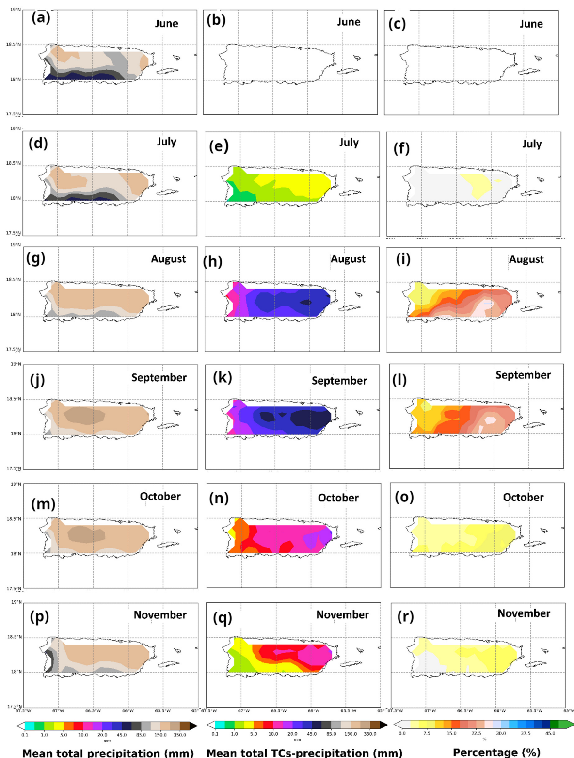
Figure 6. Mean total precipitation (a,d,g,j,m,p), Mean total TCs-precipitation (b,e,h,k,n,q) and its percentage (c,f,i,l,o,r) for June, July, August, September, October, and November. Period 1980–2016.
