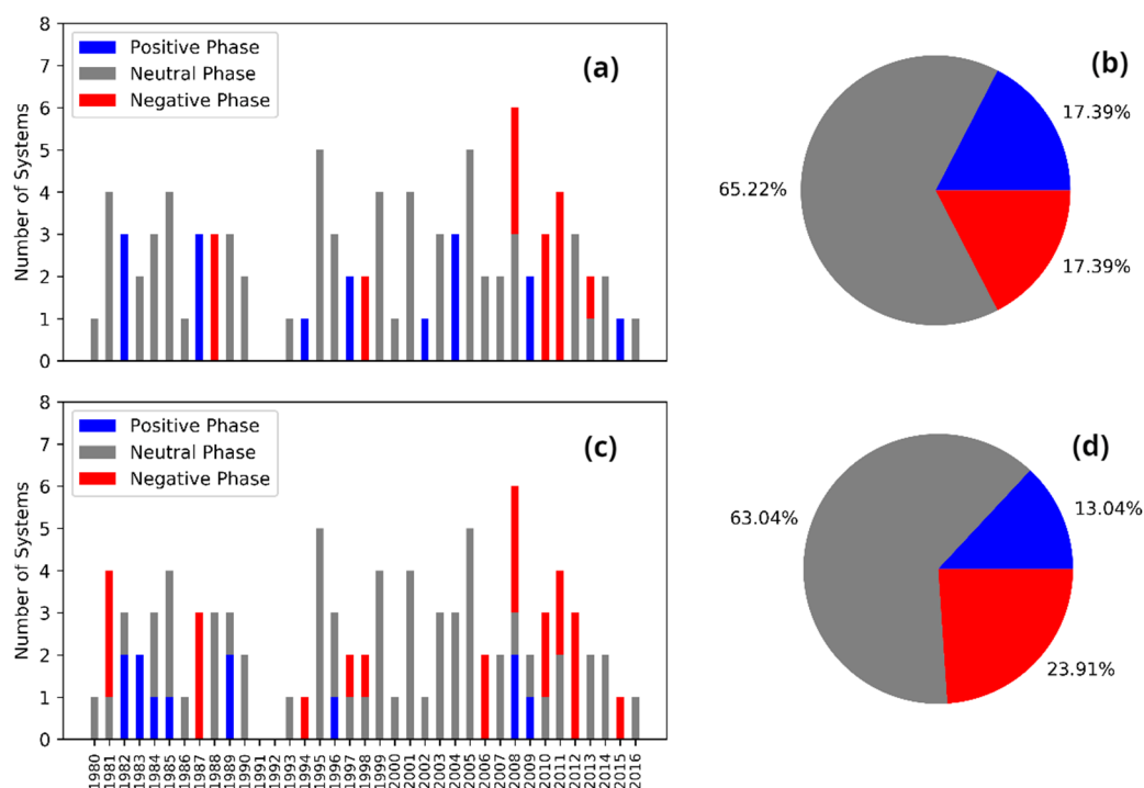
Figure 4. Left column: Number of TC systems during the different phases of ENSO (a) and NAO (c). Right column: Percentage of the number of TCs during each phase of ENSO (b), NAO (d). Period: 1980–2016.
