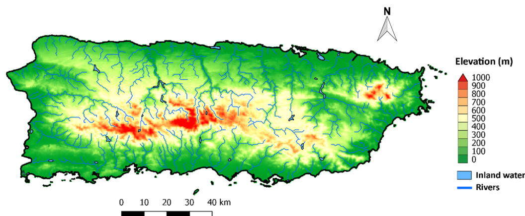
Figure 1. The geographical extension of Puerto Rico. The elevation is shaded in green-brown (in meters above sea level) from the HydroSHEDS project [28] and the river and inland water shaded in bluish colors.
