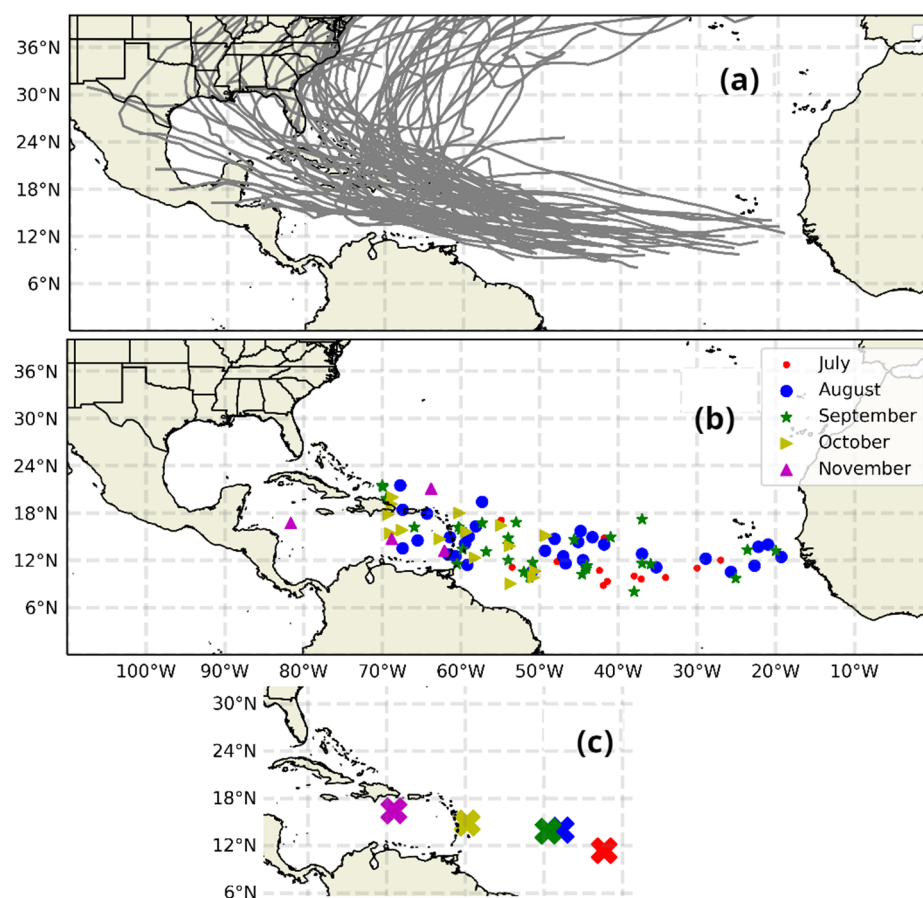
Figure 3. (a) Tracks of TCs that affected PR; (b) Areas of the genesis of TCs for the months of July to November; (c) Zoom of the mean position of genesis for each month.
