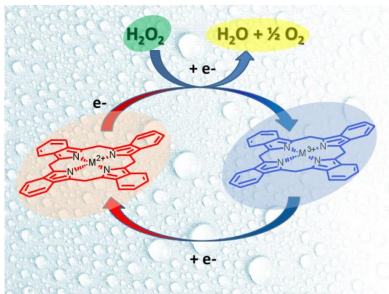
Figure 10. Peroxide electrocatalysis process mediated by MPc or MP in alkaline or neutral media.
