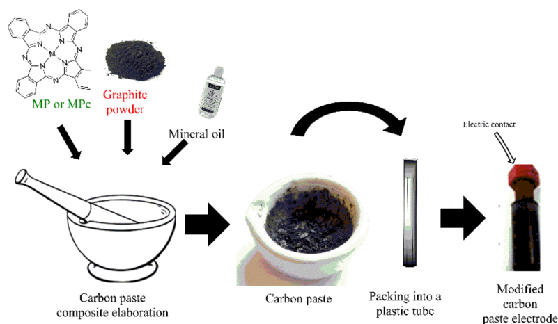
Figure 3. A simple modified CPE's elaboration process.
