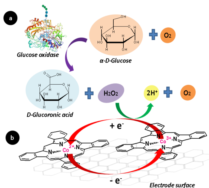
Figure 8. Basic working of an integrated bio-electrode: (a) The GOx enzyme catalyzes the oxidation of glucose and generates hydrogen peroxide as a by-product. (b) Then, the hydrogen peroxide is electro-oxidized by the metal center of the complex, and the electron exchange of the reaction is used in an electroanalytical technique to quantify the amount of glucose in a sample.
